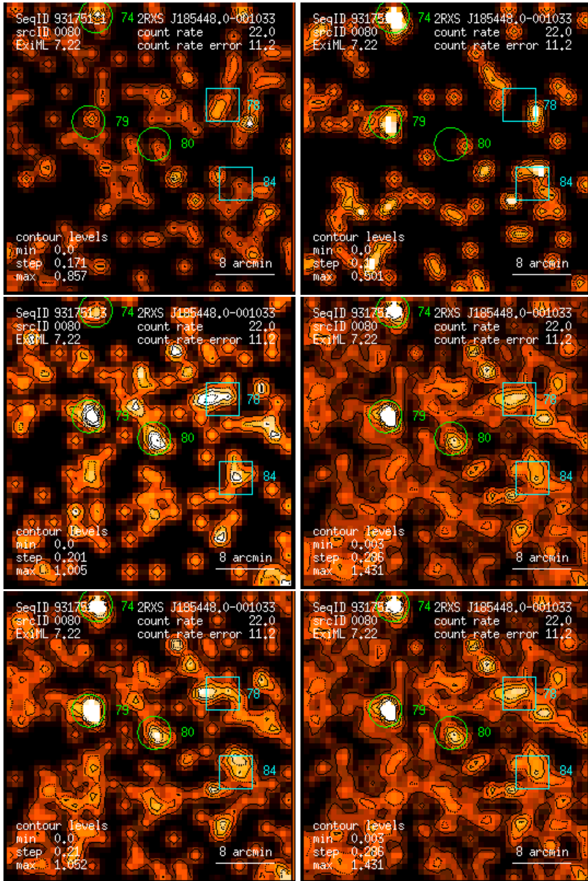
Figure 80: RASS 931751: detection 0080: band rate images, Gaussian filter: (1) PSPC channels 11 – 41, (2) 52 – 90, (3) 91 – 201, (4) 11 – 235, (5) 52 – 201, (6) 11 – 201. Broad band rates in counts/ks. Band rate contour levels in counts/ks/arcmin 2 .
