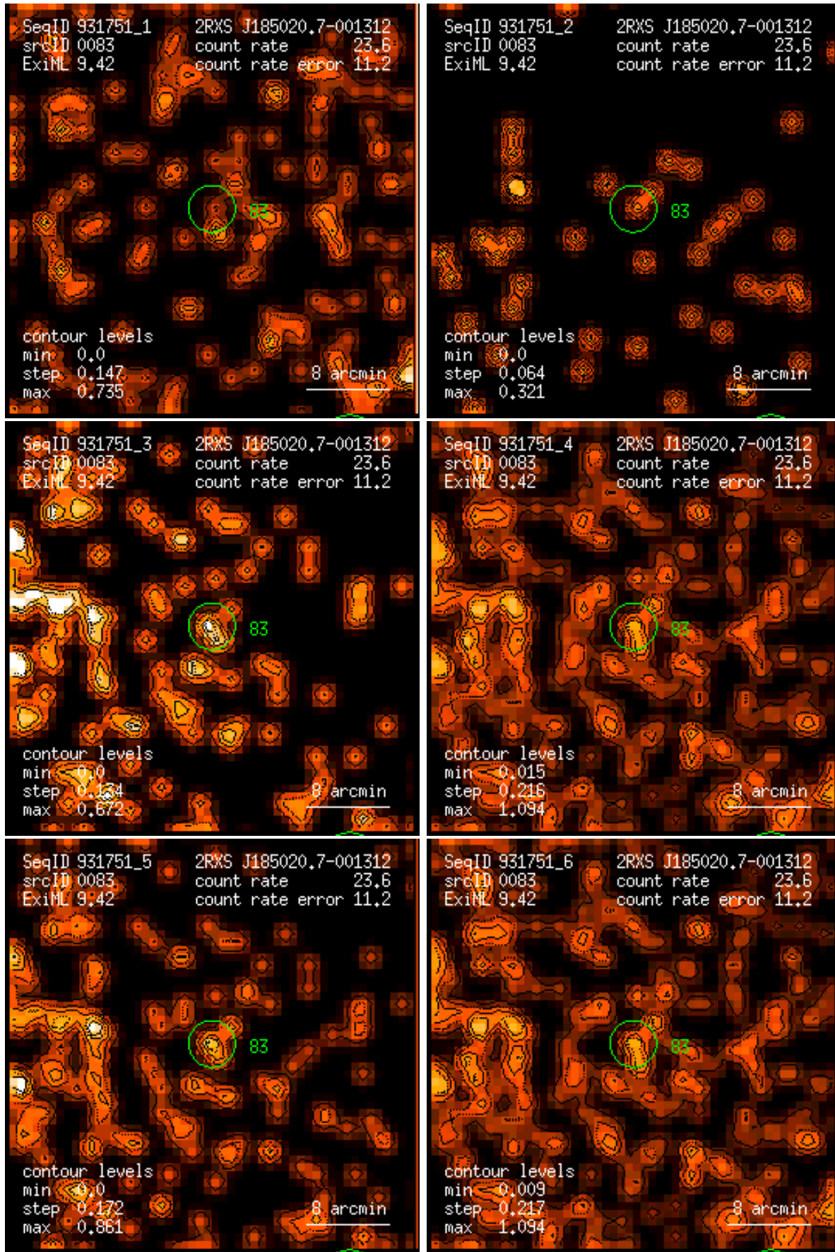
Figure 83: RASS 931751: detection 0083: band rate images, Gaussian filter: (1) PSPC channels 11 – 41, (2) 52 – 90, (3) 91 – 201, (4) 11 – 235, (5) 52 – 201, (6) 11 – 201. Broad band rates in counts/ks. Band rate contour levels in counts/ks/arcmin 2 .
