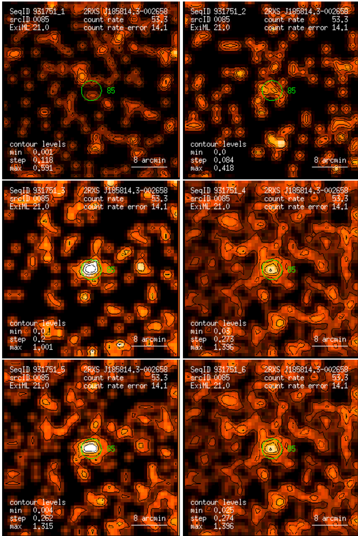
Figure 85: RASS 931751: detection 0085: band rate images, Gaussian filter: (1) PSPC channels 11 – 41, (2) 52 – 90, (3) 91 – 201, (4) 11 – 235, (5) 52 – 201, (6) 11 – 201. Broad band rates in counts/ks. Band rate contour levels in counts/ks/arcmin 2 .
