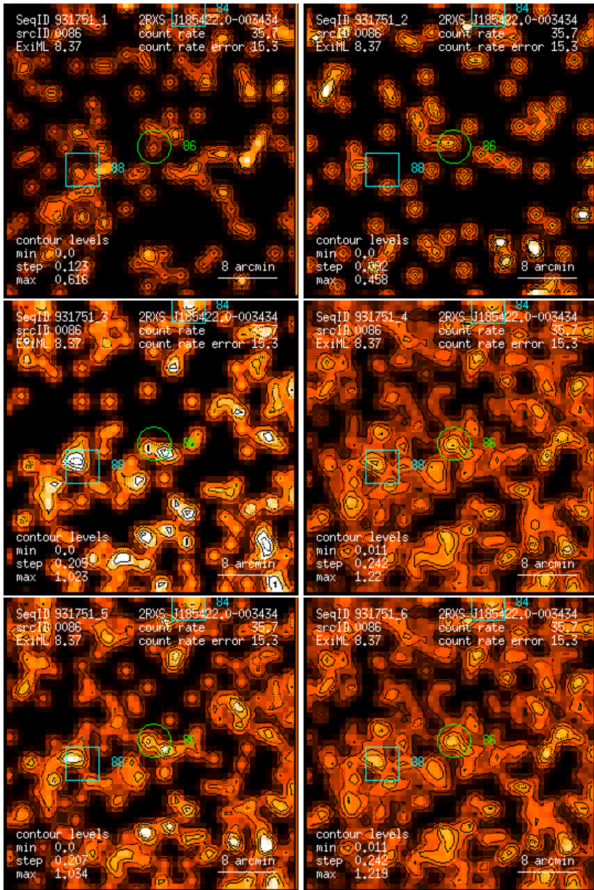
Figure 86: RASS 931751: detection 0086: band rate images, Gaussian filter: (1) PSPC channels 11 – 41, (2) 52 – 90, (3) 91 – 201, (4) 11 – 235, (5) 52 – 201, (6) 11 – 201. Broad band rates in counts/ks. Band rate contour levels in counts/ks/arcmin 2 .
