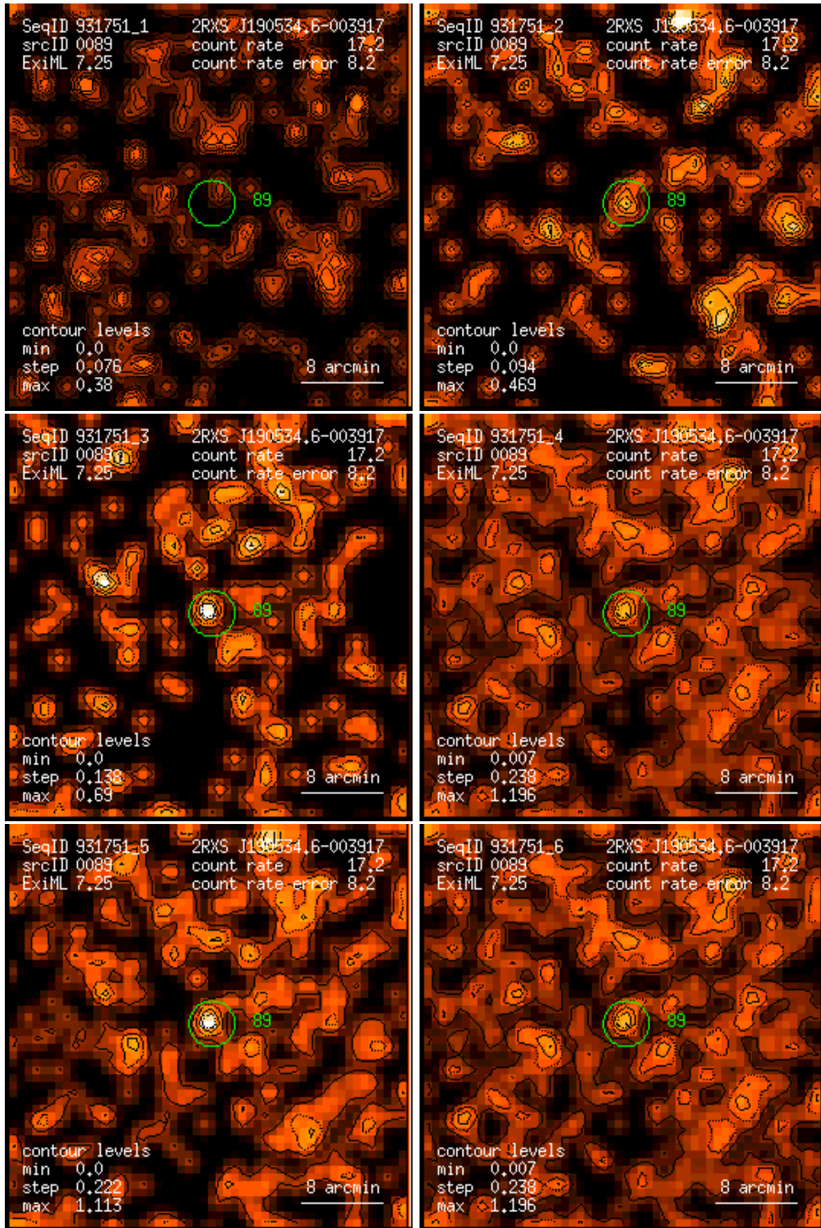
Figure 89: RASS 931751: detection 0089: band rate images, Gaussian filter: (1) PSPC channels 11 – 41, (2) 52 – 90, (3) 91 – 201, (4) 11 – 235, (5) 52 – 201, (6) 11 – 201. Broad band rates in counts/ks. Band rate contour levels in counts/ks/arcmin 2 .
