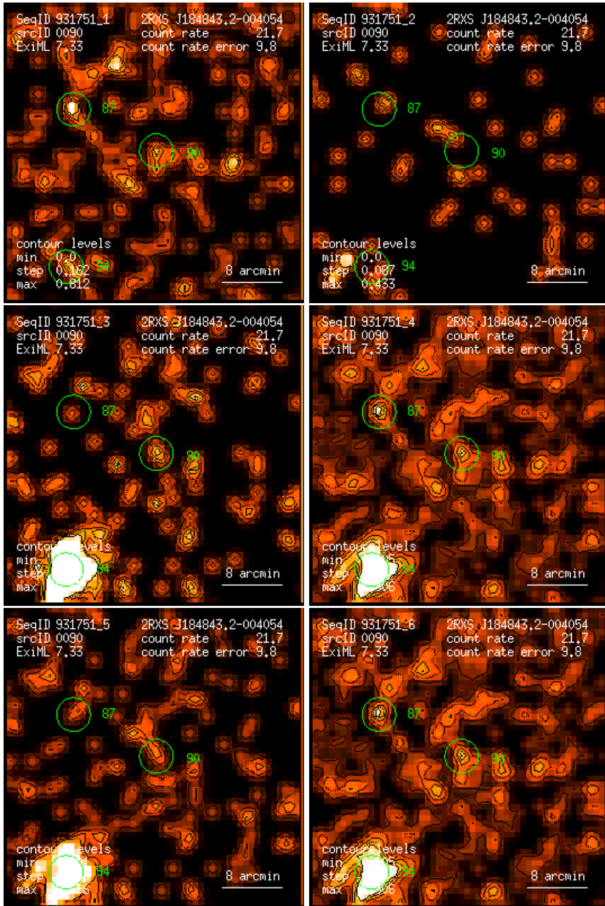
Figure 90: RASS 931751: detection 0090: band rate images, Gaussian filter: (1) PSPC channels 11 – 41, (2) 52 – 90, (3) 91 – 201, (4) 11 – 235, (5) 52 – 201, (6) 11 – 201. Broad band rates in counts/ks. Band rate contour levels in counts/ks/arcmin 2 .
