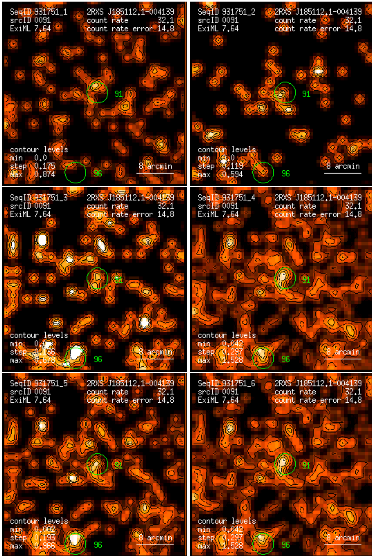
Figure 91: RASS 931751: detection 0091: band rate images, Gaussian filter: (1) PSPC channels 11 – 41, (2) 52 – 90, (3) 91 – 201, (4) 11 – 235, (5) 52 – 201, (6) 11 – 201. Broad band rates in counts/ks. Band rate contour levels in counts/ks/arcmin 2 .
