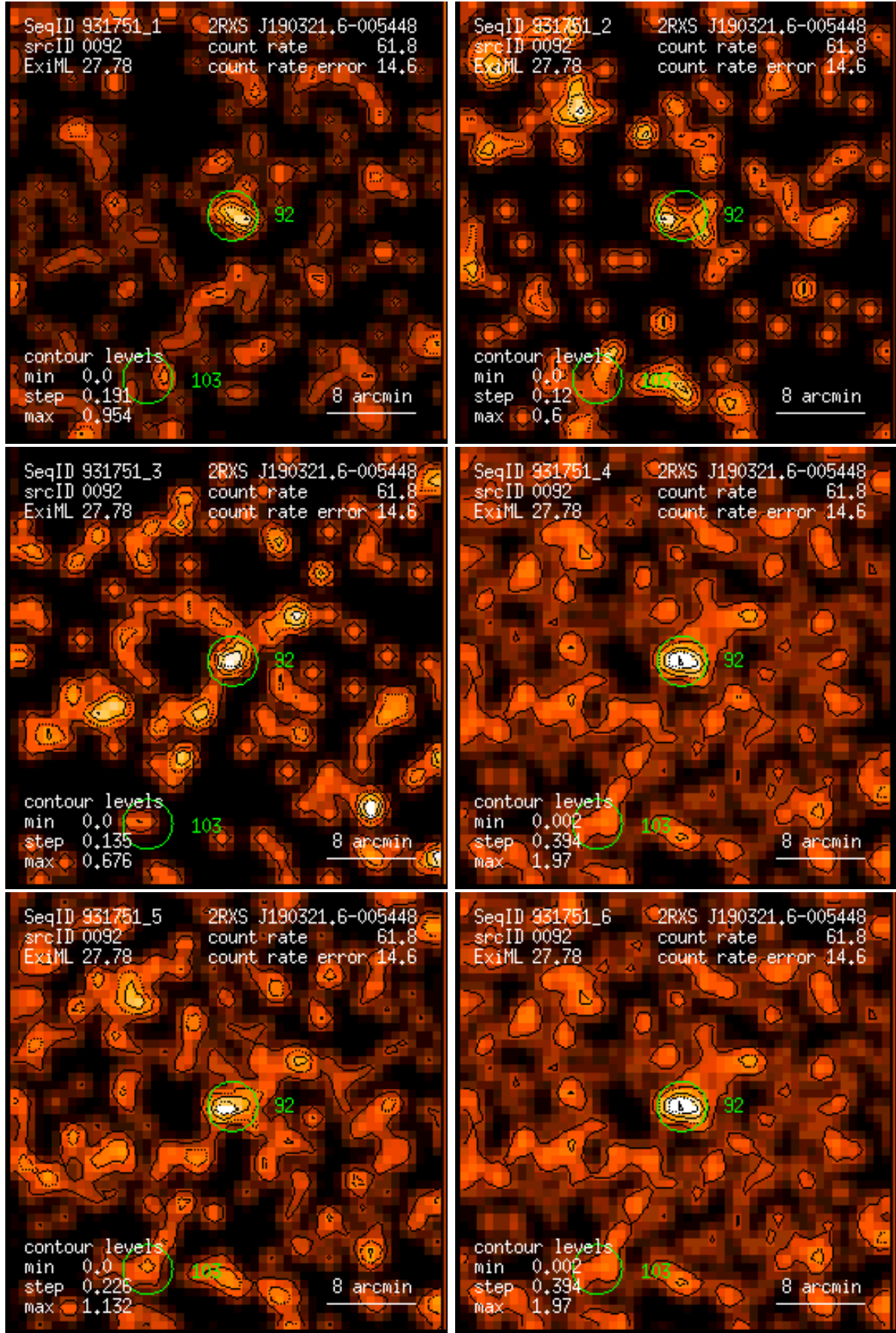
Figure 92: RASS 931751: detection 0092: band rate images, Gaussian filter: (1) PSPC channels 11 – 41, (2) 52 – 90, (3) 91 – 201, (4) 11 – 235, (5) 52 – 201, (6) 11 – 201. Broad band rates in counts/ks. Band rate contour levels in counts/ks/arcmin 2 .
