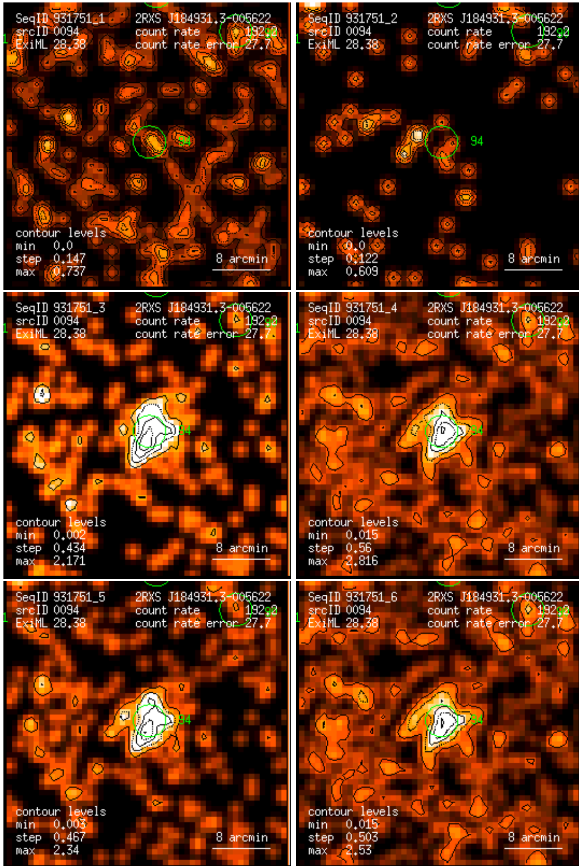
Figure 94: RASS 931751: detection 0094: band rate images, Gaussian filter: (1) PSPC channels 11 – 41, (2) 52 – 90, (3) 91 – 201, (4) 11 – 235, (5) 52 – 201, (6) 11 – 201. Broad band rates in counts/ks. Band rate contour levels in counts/ks/arcmin 2 .
