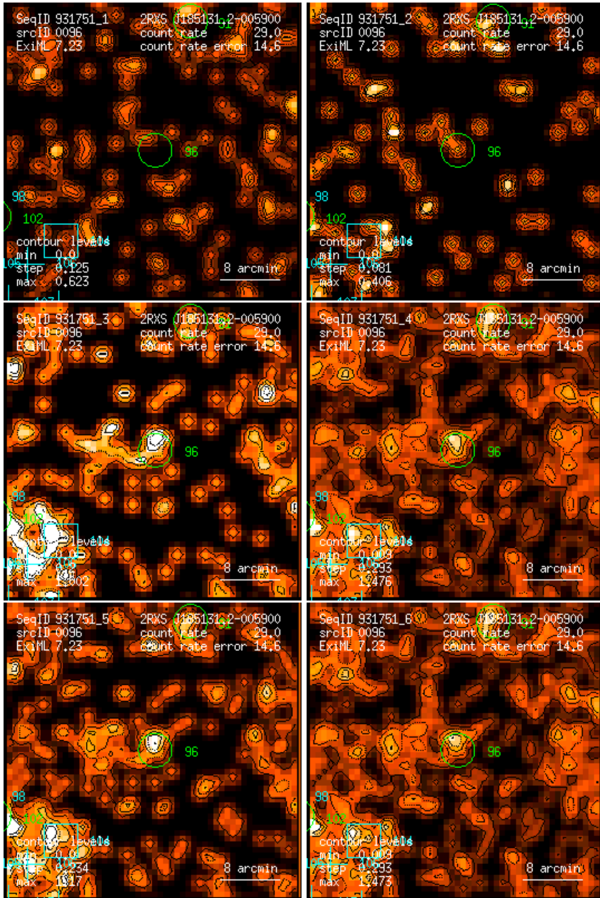
Figure 96: RASS 931751: detection 0096: band rate images, Gaussian filter: (1) PSPC channels 11 – 41, (2) 52 – 90, (3) 91 – 201, (4) 11 – 235, (5) 52 – 201, (6) 11 – 201. Broad band rates in counts/ks. Band rate contour levels in counts/ks/arcmin 2 .
