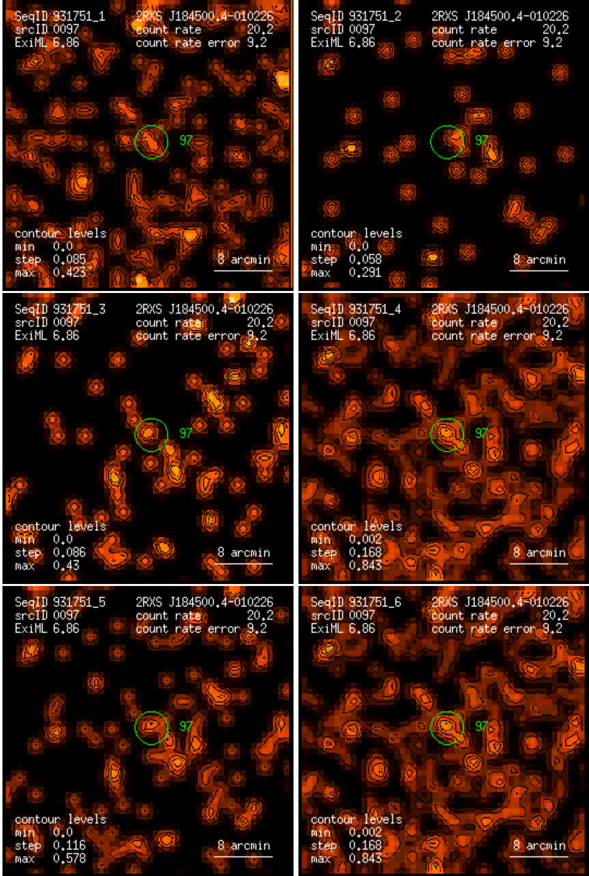
Figure 97: RASS 931751: detection 0097: band rate images, Gaussian filter: (1) PSPC channels 11 – 41, (2) 52 – 90, (3) 91 – 201, (4) 11 – 235, (5) 52 – 201, (6) 11 – 201. Broad band rates in counts/ks. Band rate contour levels in counts/ks/arcmin 2 .
