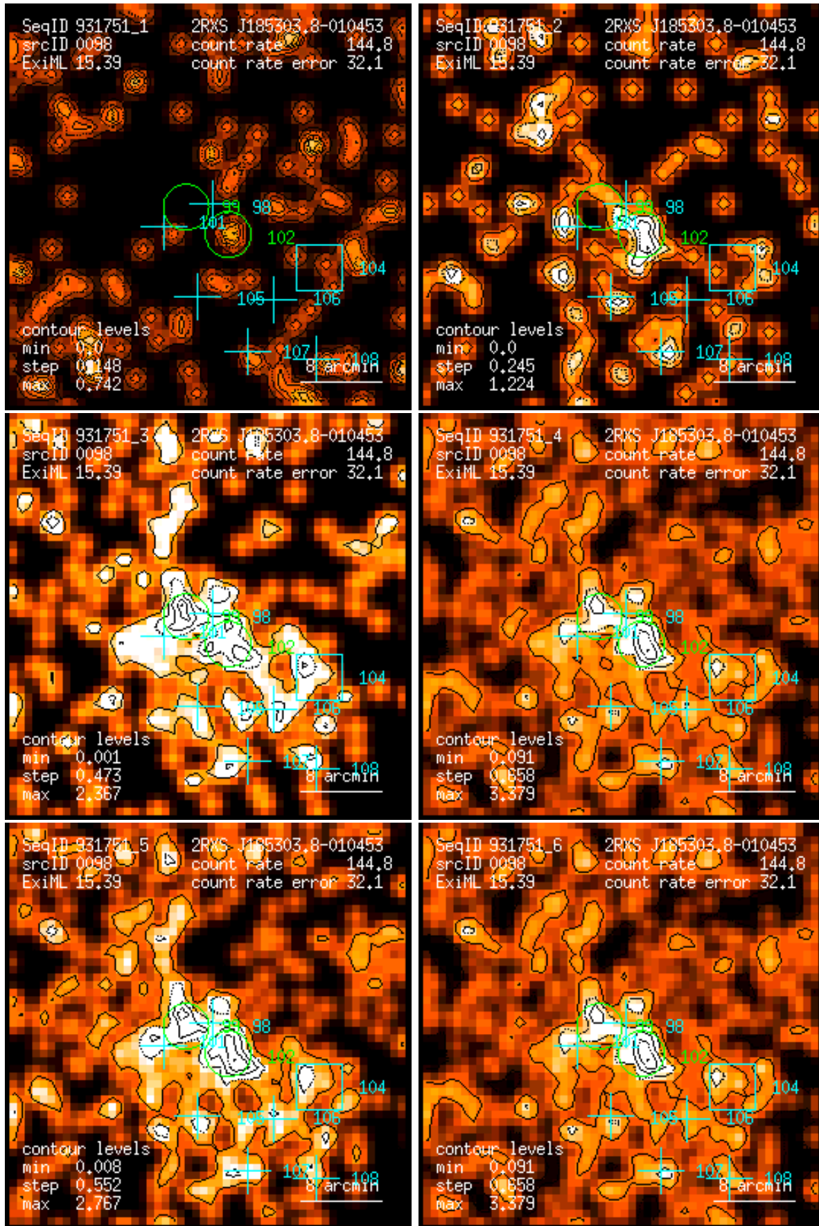
Figure 98: RASS 931751: detection 0098: band rate images, Gaussian filter: (1) PSPC channels 11 – 41, (2) 52 – 90, (3) 91 – 201, (4) 11 – 235, (5) 52 – 201, (6) 11 – 201. Broad band rates in counts/ks. Band rate contour levels in counts/ks/arcmin 2 .
