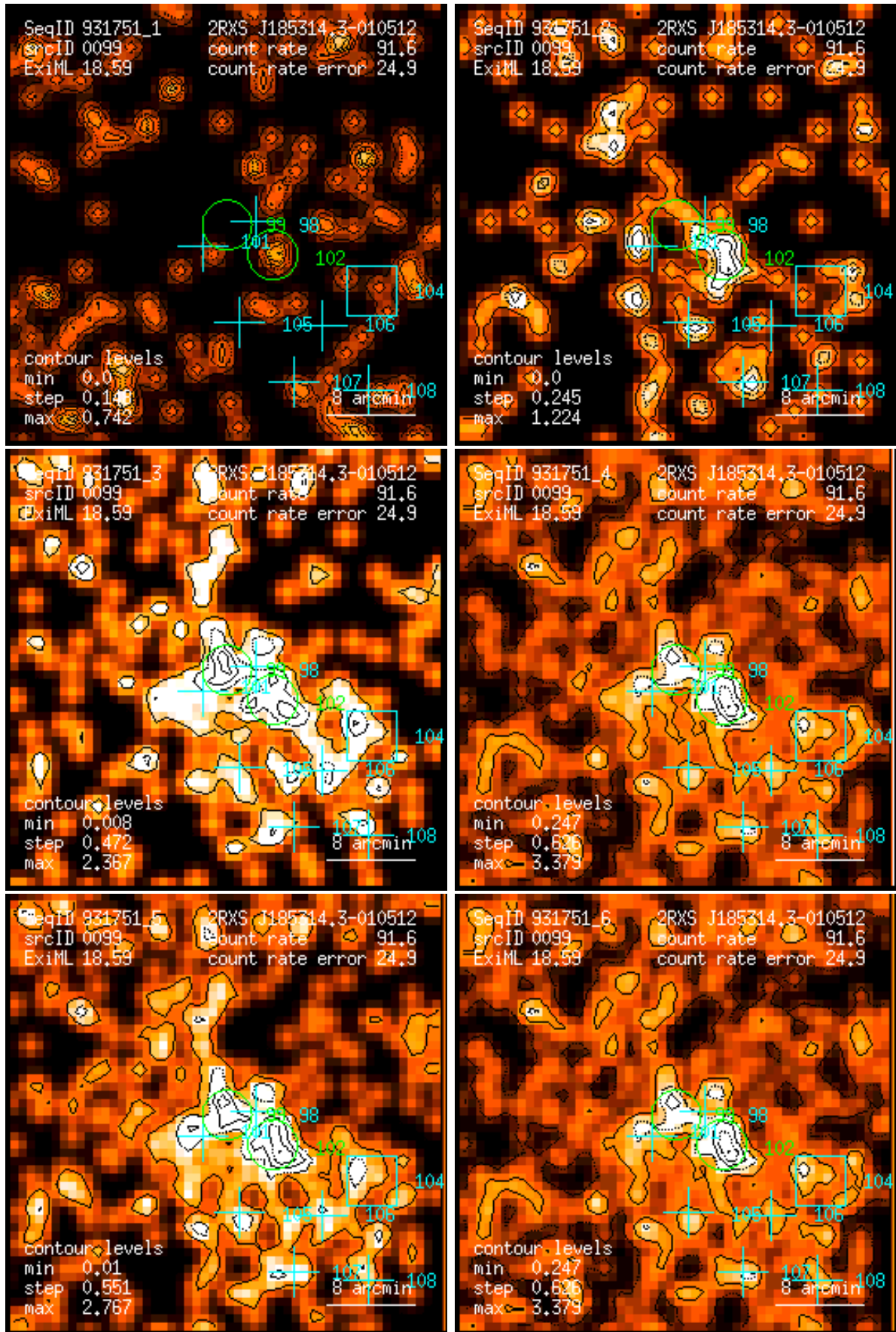
Figure 99: RASS 931751: detection 0099: band rate images, Gaussian filter: (1) PSPC channels 11 – 41, (2) 52 – 90, (3) 91 – 201, (4) 11 – 235, (5) 52 – 201, (6) 11 – 201. Broad band rates in counts/ks. Band rate contour levels in counts/ks/arcmin 2 .
