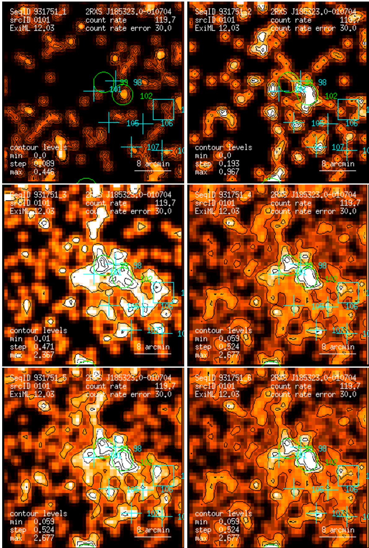
Figure 101: RASS 931751: detection 0101: band rate images, Gaussian filter: (1) PSPC channels 11 – 41, (2) 52 – 90, (3) 91 – 201, (4) 11 – 235, (5) 52 – 201, (6) 11 – 201. Broad band rates in counts/ks. Band rate contour levels in counts/ks/arcmin 2 .
