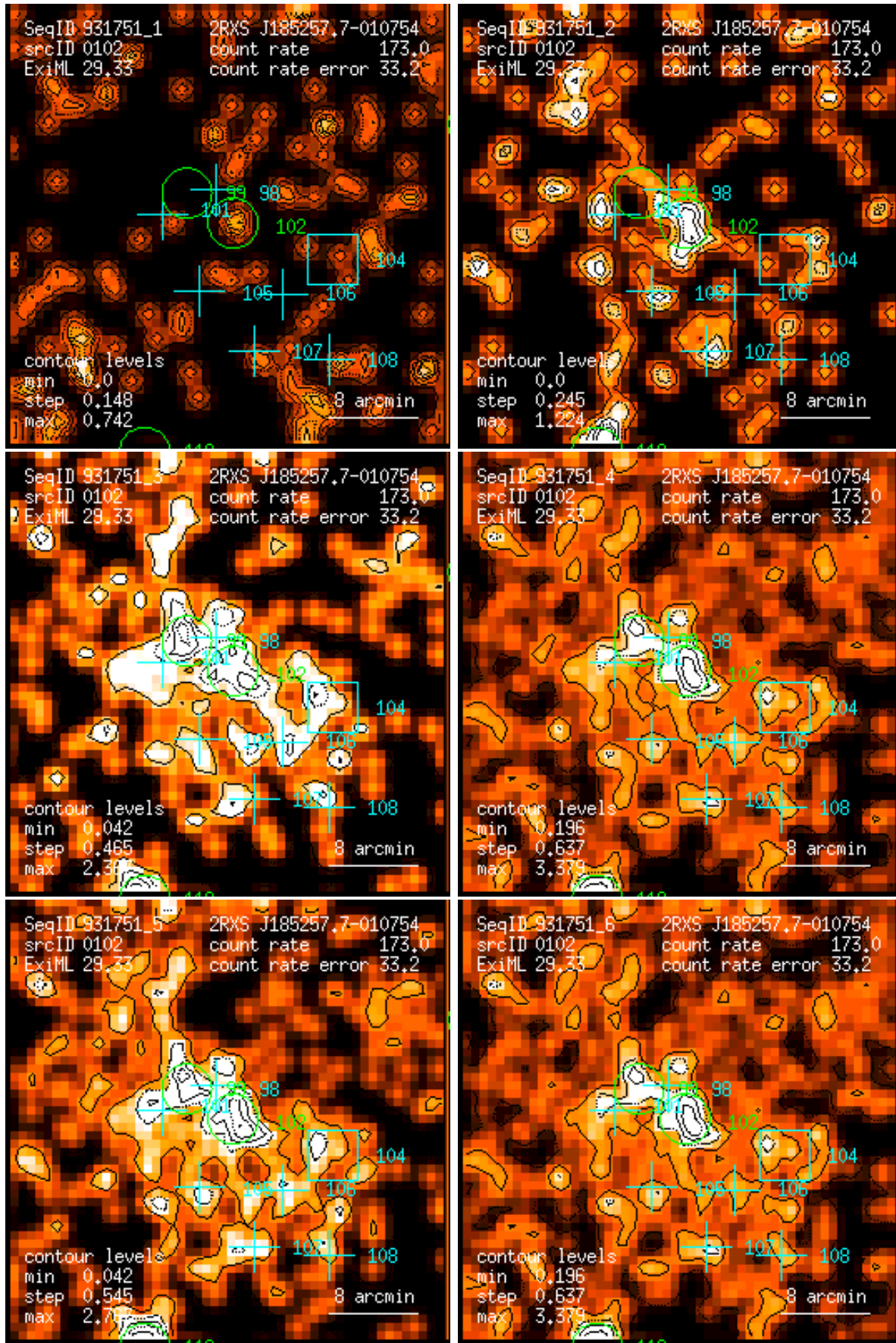
Figure 102: RASS 931751: detection 0102: band rate images, Gaussian filter: (1) PSPC channels 11 – 41, (2) 52 – 90, (3) 91 – 201, (4) 11 – 235, (5) 52 – 201, (6) 11 – 201. Broad band rates in counts/ks. Band rate contour levels in counts/ks/arcmin 2 .
