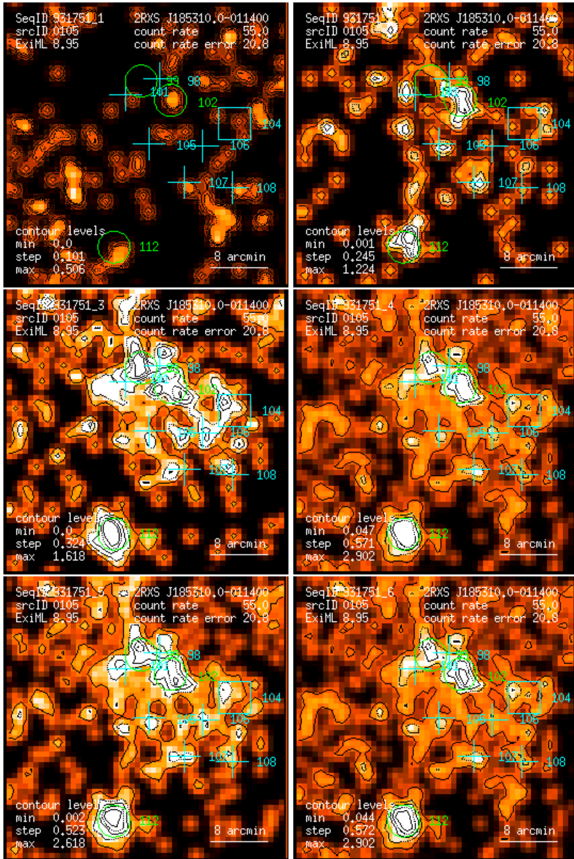
Figure 105: RASS 931751: detection 0105: band rate images, Gaussian filter: (1) PSPC channels 11 – 41, (2) 52 – 90, (3) 91 – 201, (4) 11 – 235, (5) 52 – 201, (6) 11 – 201. Broad band rates in counts/ks. Band rate contour levels in counts/ks/arcmin 2 .
