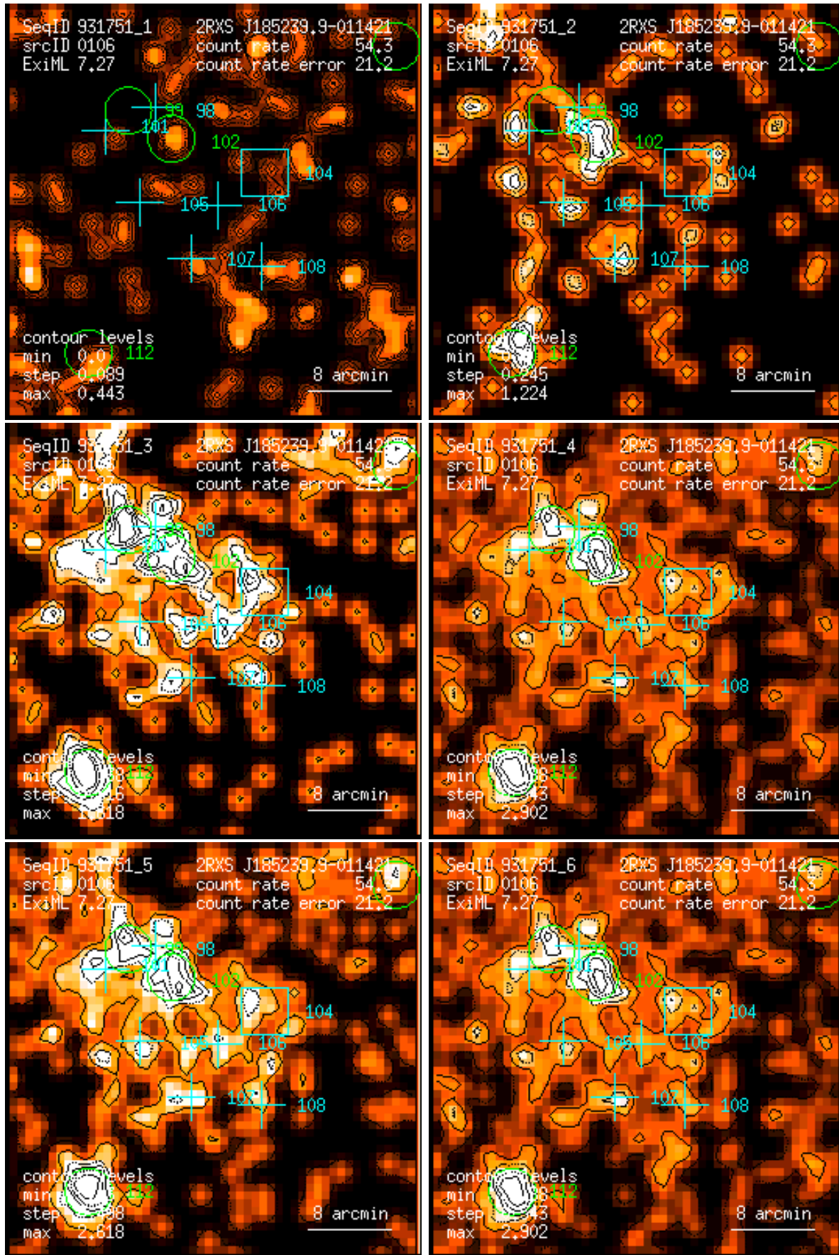
Figure 106: RASS 931751: detection 0106: band rate images, Gaussian filter: (1) PSPC channels 11 – 41, (2) 52 – 90, (3) 91 – 201, (4) 11 – 235, (5) 52 – 201, (6) 11 – 201. Broad band rates in counts/ks. Band rate contour levels in counts/ks/arcmin 2 .
