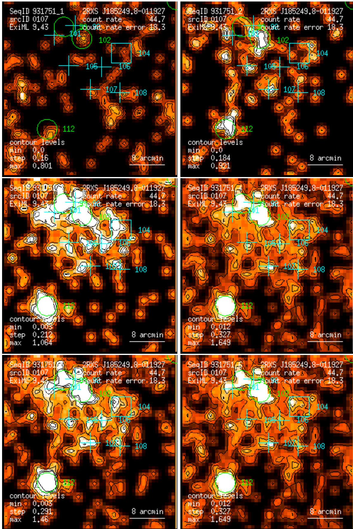
Figure 107: RASS 931751: detection 0107: band rate images, Gaussian filter: (1) PSPC channels 11 – 41, (2) 52 – 90, (3) 91 – 201, (4) 11 – 235, (5) 52 – 201, (6) 11 – 201. Broad band rates in counts/ks. Band rate contour levels in counts/ks/arcmin 2 .
