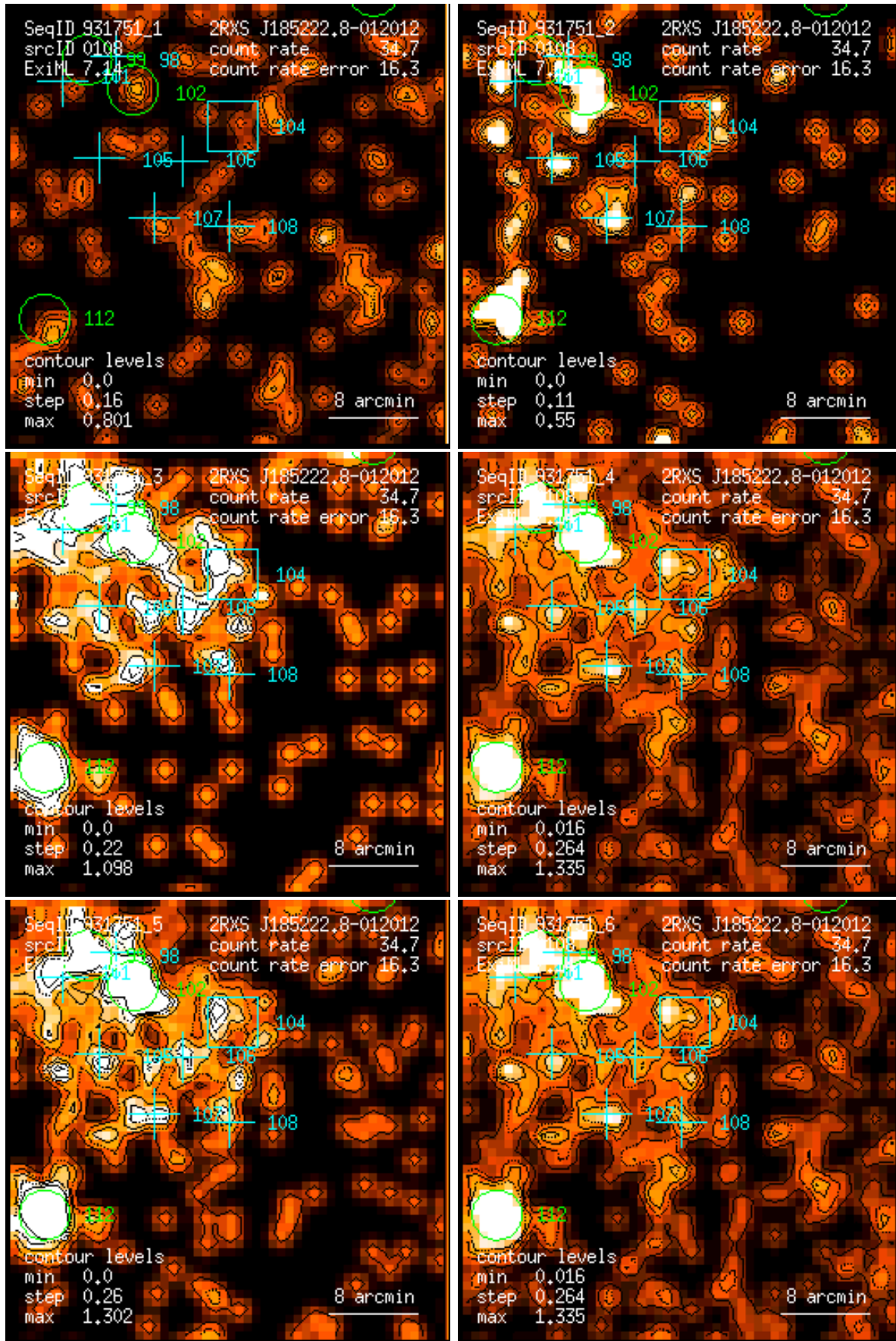
Figure 108: RASS 931751: detection 0108: band rate images, Gaussian filter: (1) PSPC channels 11 – 41, (2) 52 – 90, (3) 91 – 201, (4) 11 – 235, (5) 52 – 201, (6) 11 – 201. Broad band rates in counts/ks. Band rate contour levels in counts/ks/arcmin 2 .
