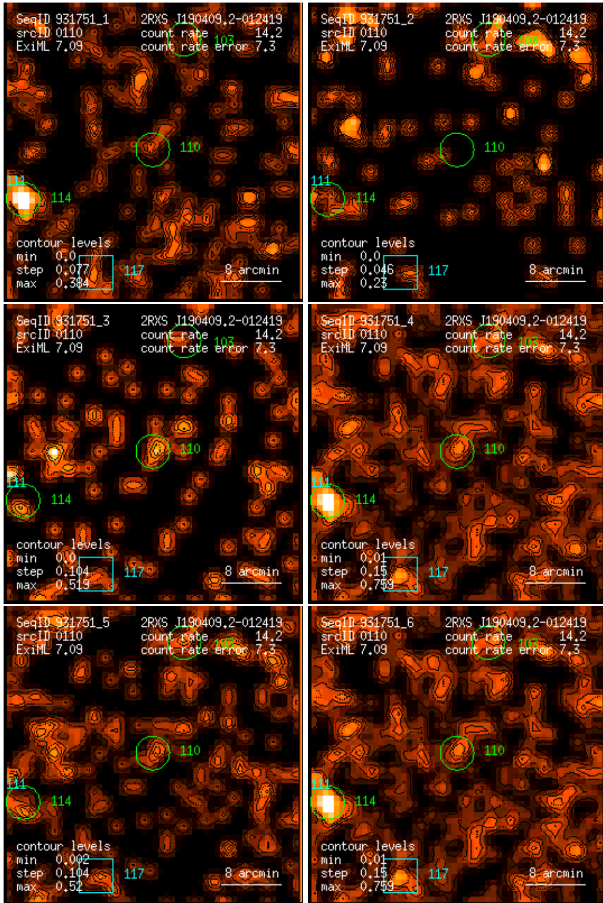
Figure 110: RASS 931751: detection 0110: band rate images, Gaussian filter: (1) PSPC channels 11 – 41, (2) 52 – 90, (3) 91 – 201, (4) 11 – 235, (5) 52 – 201, (6) 11 – 201. Broad band rates in counts/ks. Band rate contour levels in counts/ks/arcmin 2 .
