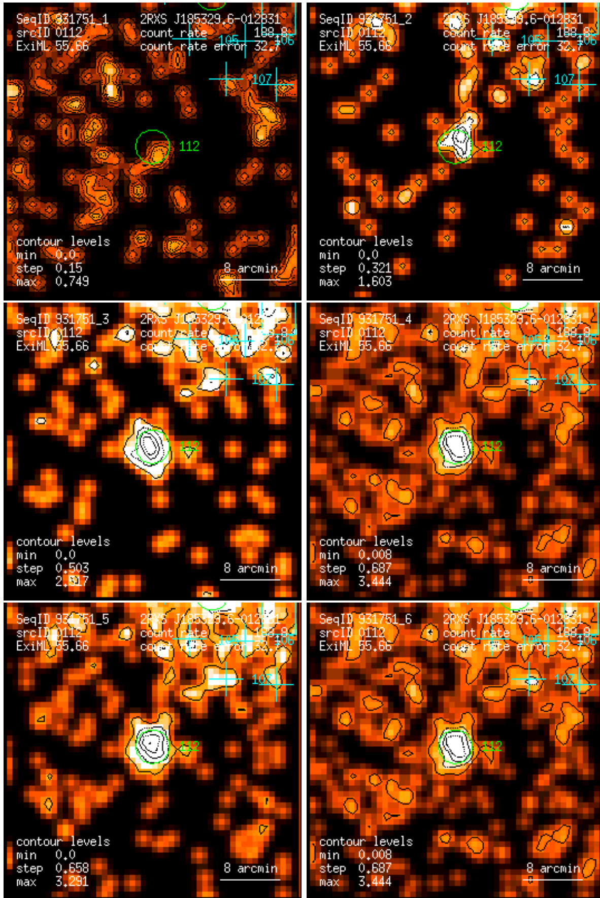
Figure 112: RASS 931751: detection 0112: band rate images, Gaussian filter: (1) PSPC channels 11 – 41, (2) 52 – 90, (3) 91 – 201, (4) 11 – 235, (5) 52 – 201, (6) 11 – 201. Broad band rates in counts/ks. Band rate contour levels in counts/ks/arcmin 2 .
