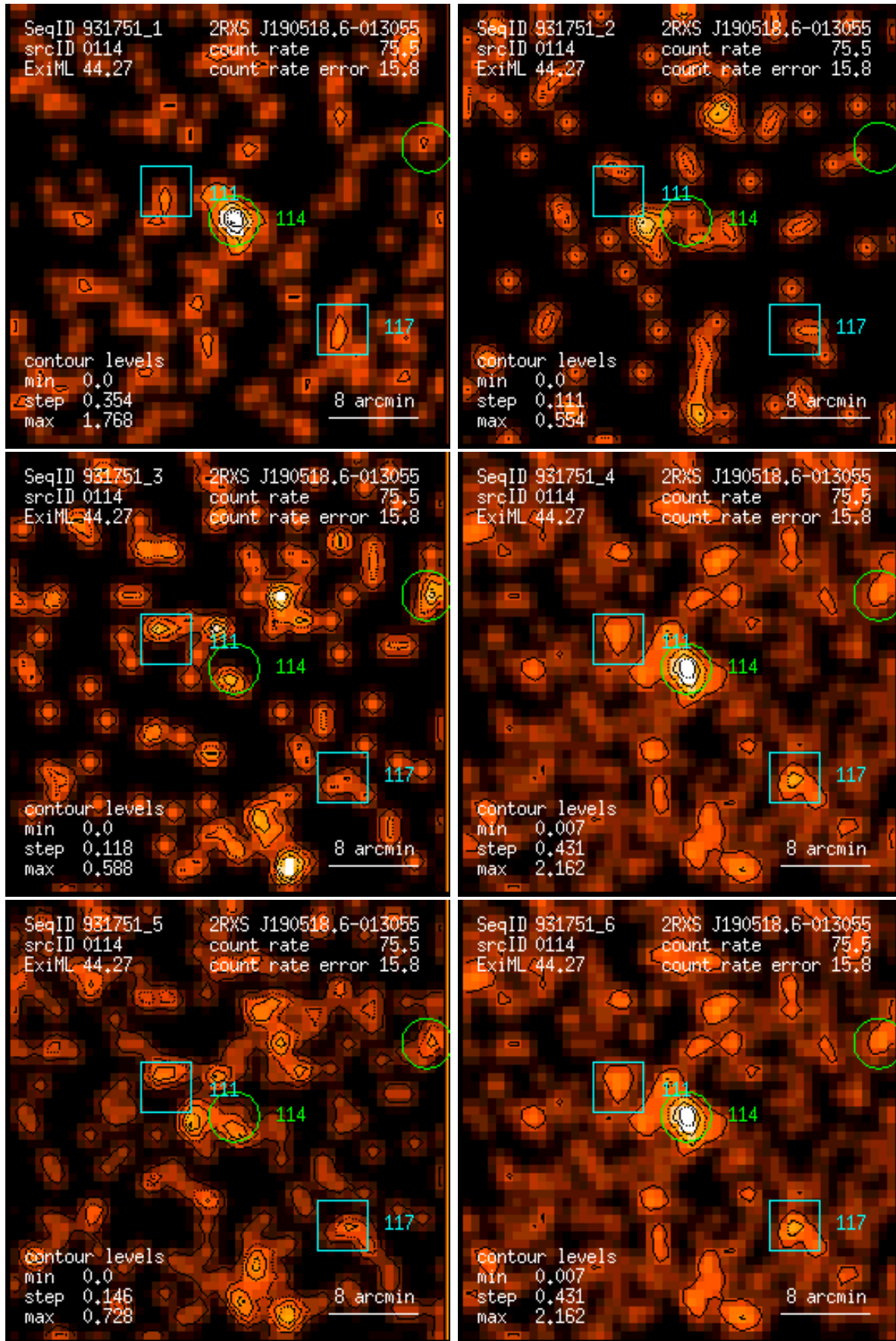
Figure 114: RASS 931751: detection 0114: band rate images, Gaussian filter: (1) PSPC channels 11 – 41, (2) 52 – 90, (3) 91 – 201, (4) 11 – 235, (5) 52 – 201, (6) 11 – 201. Broad band rates in counts/ks. Band rate contour levels in counts/ks/arcmin 2 .
