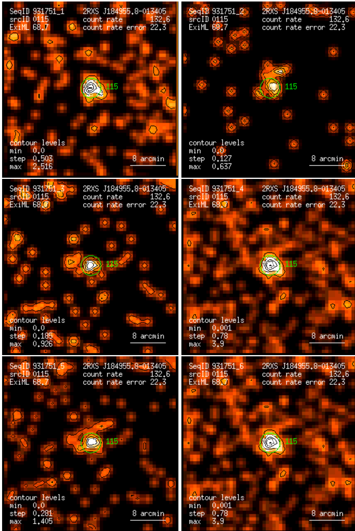
Figure 115: RASS 931751: detection 0115: band rate images, Gaussian filter: (1) PSPC channels 11 – 41, (2) 52 – 90, (3) 91 – 201, (4) 11 – 235, (5) 52 – 201, (6) 11 – 201. Broad band rates in counts/ks. Band rate contour levels in counts/ks/arcmin 2 .
