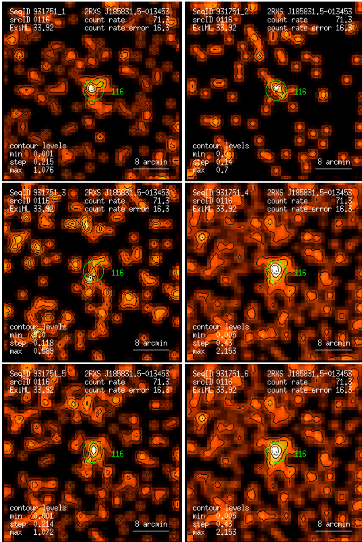
Figure 116: RASS 931751: detection 0116: band rate images, Gaussian filter: (1) PSPC channels 11 – 41, (2) 52 – 90, (3) 91 – 201, (4) 11 – 235, (5) 52 – 201, (6) 11 – 201. Broad band rates in counts/ks. Band rate contour levels in counts/ks/arcmin 2 .
