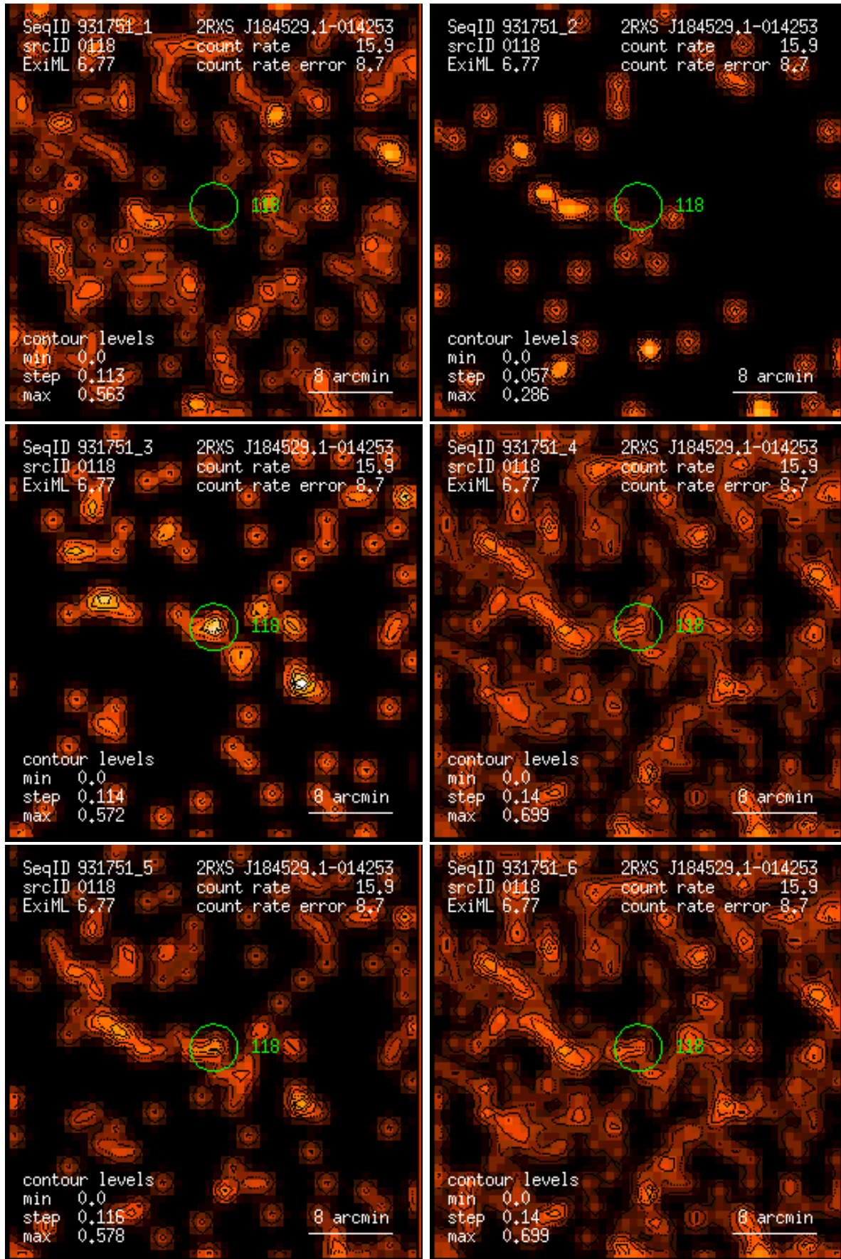
Figure 118: RASS 931751: detection 0118: band rate images, Gaussian filter: (1) PSPC channels 11 – 41, (2) 52 – 90, (3) 91 – 201, (4) 11 – 235, (5) 52 – 201, (6) 11 – 201. Broad band rates in counts/ks. Band rate contour levels in counts/ks/arcmin 2 .
