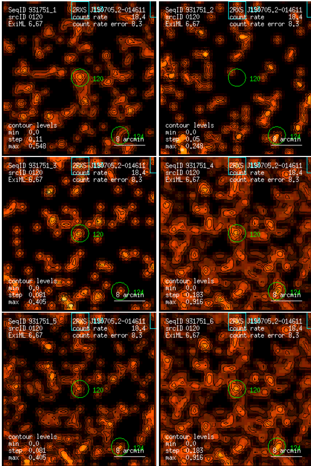
Figure 120: RASS 931751: detection 0120: band rate images, Gaussian filter: (1) PSPC channels 11 – 41, (2) 52 – 90, (3) 91 – 201, (4) 11 – 235, (5) 52 – 201, (6) 11 – 201. Broad band rates in counts/ks. Band rate contour levels in counts/ks/arcmin 2 .
