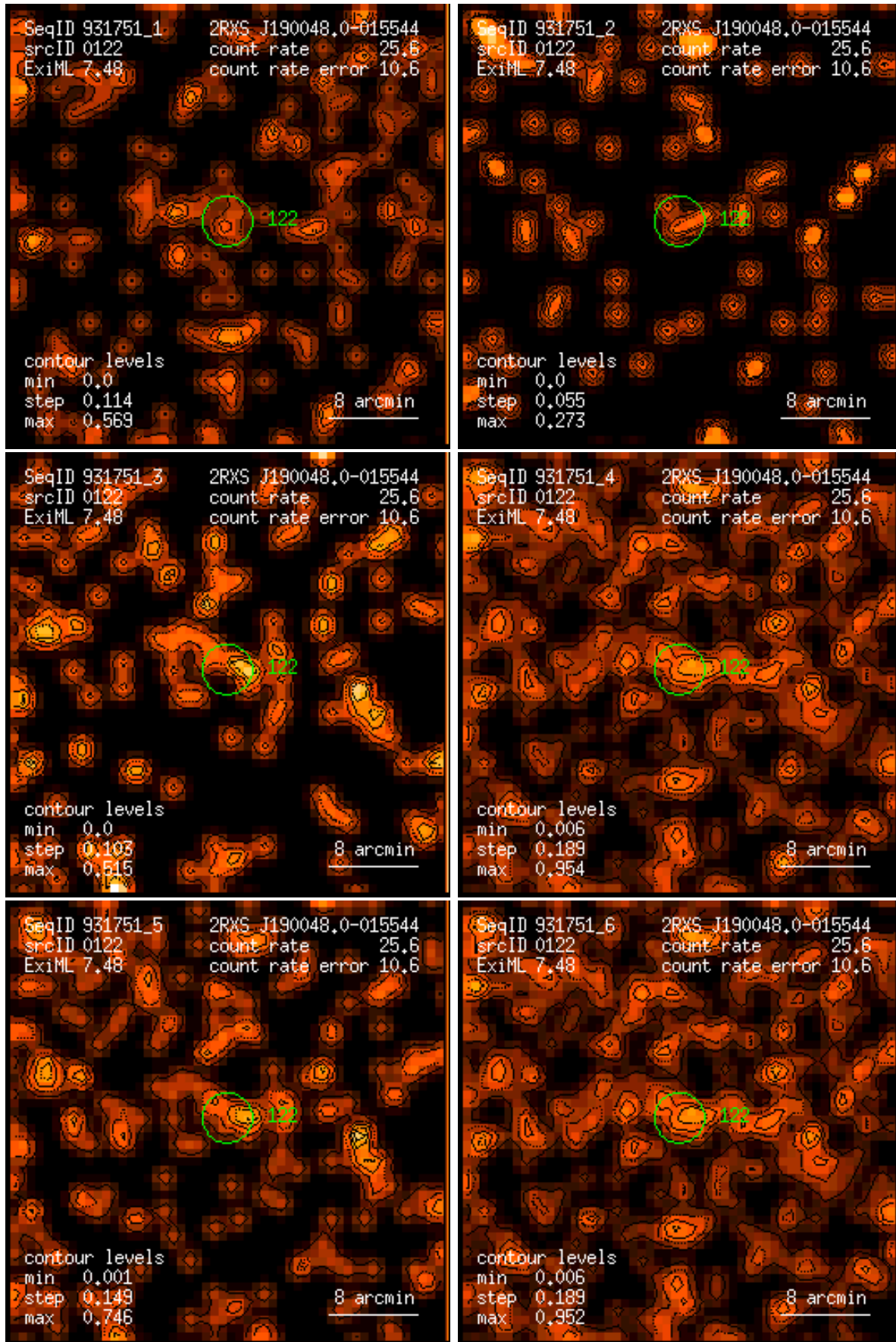
Figure 122: RASS 931751: detection 0122: band rate images, Gaussian filter: (1) PSPC channels 11 – 41, (2) 52 – 90, (3) 91 – 201, (4) 11 – 235, (5) 52 – 201, (6) 11 – 201. Broad band rates in counts/ks. Band rate contour levels in counts/ks/arcmin 2 .
