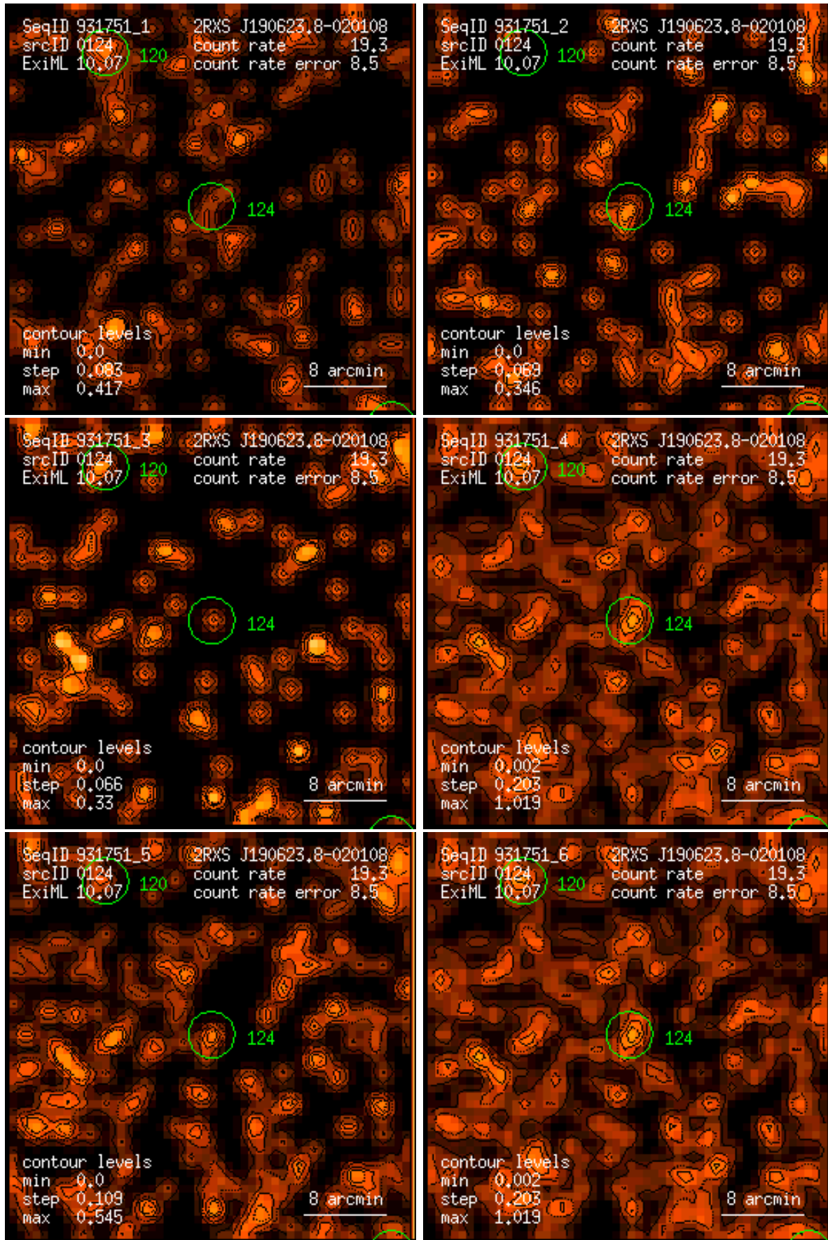
Figure 124: RASS 931751: detection 0124: band rate images, Gaussian filter: (1) PSPC channels 11 – 41, (2) 52 – 90, (3) 91 – 201, (4) 11 – 235, (5) 52 – 201, (6) 11 – 201. Broad band rates in counts/ks. Band rate contour levels in counts/ks/arcmin 2 .
