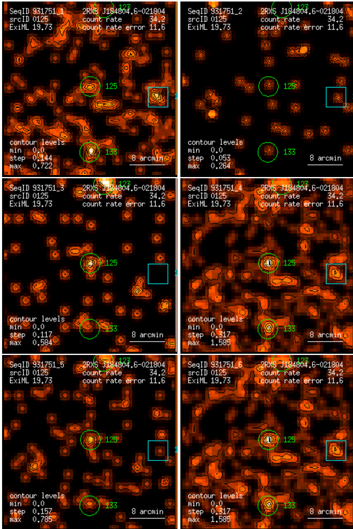
Figure 125: RASS 931751: detection 0125: band rate images, Gaussian filter: (1) PSPC channels 11 – 41, (2) 52 – 90, (3) 91 – 201, (4) 11 – 235, (5) 52 – 201, (6) 11 – 201. Broad band rates in counts/ks. Band rate contour levels in counts/ks/arcmin 2 .
