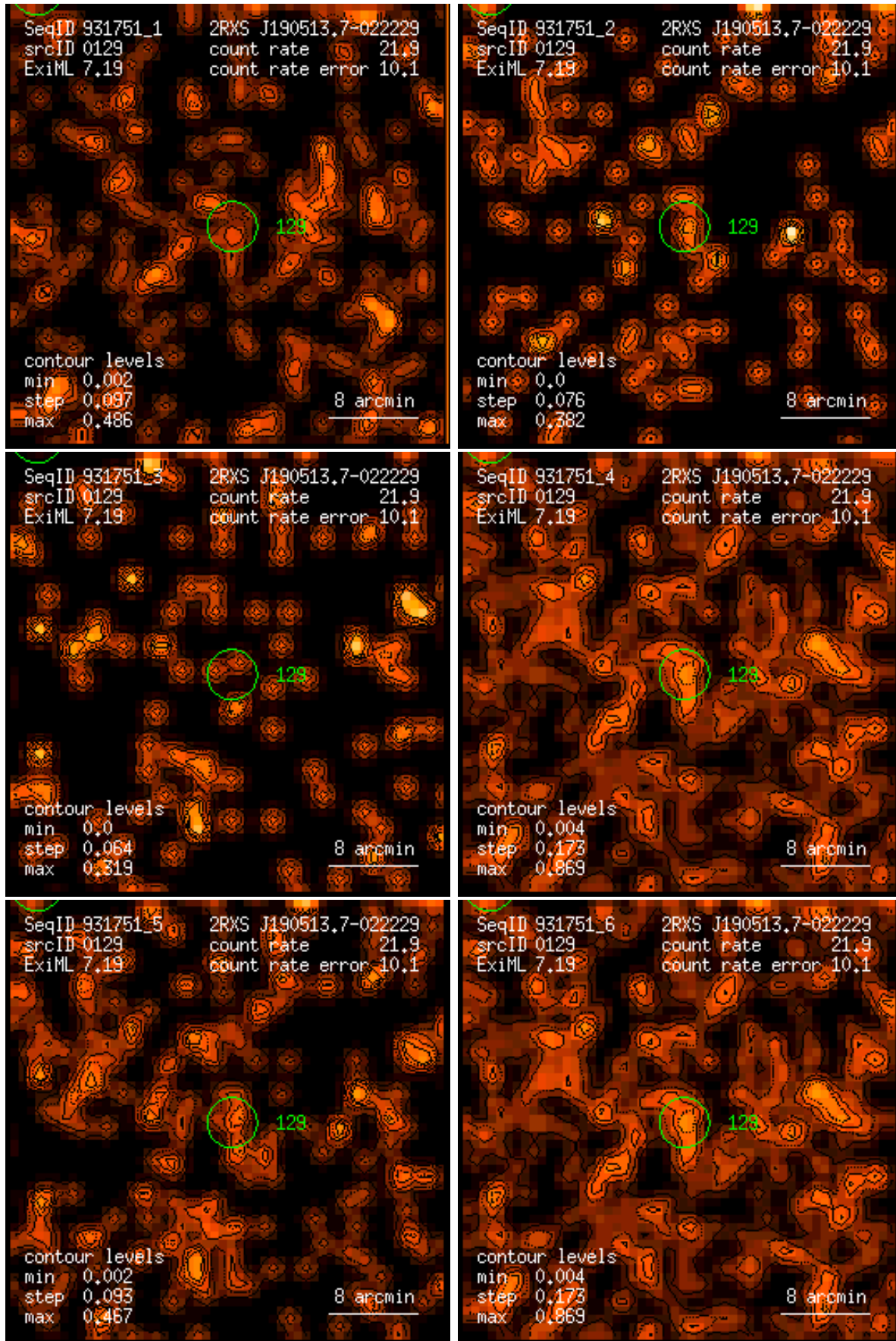
Figure 129: RASS 931751: detection 0129: band rate images, Gaussian filter: (1) PSPC channels 11 – 41, (2) 52 – 90, (3) 91 – 201, (4) 11 – 235, (5) 52 – 201, (6) 11 – 201. Broad band rates in counts/ks. Band rate contour levels in counts/ks/arcmin 2 .
