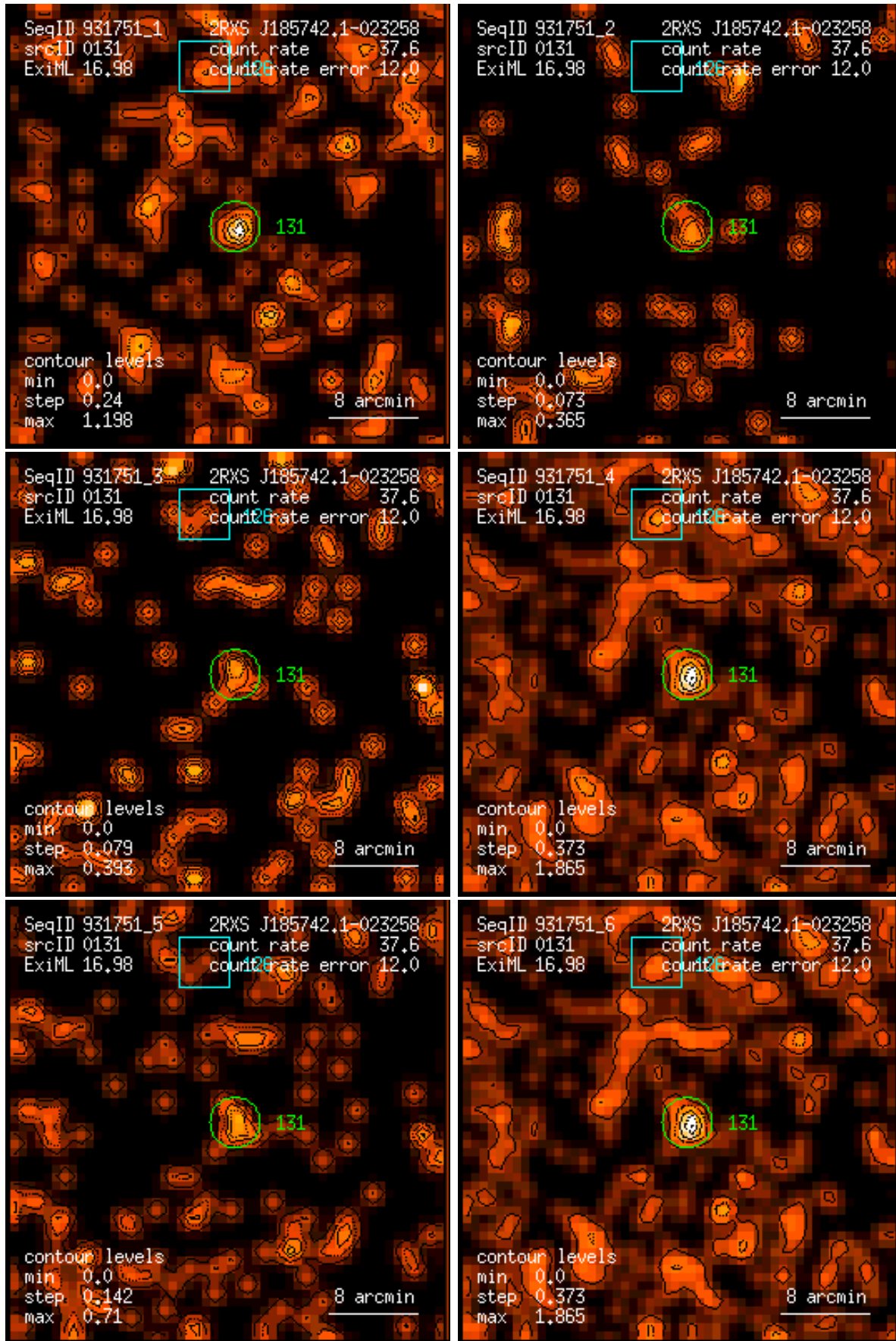
Figure 131: RASS 931751: detection 0131: band rate images, Gaussian filter: (1) PSPC channels 11 – 41, (2) 52 – 90, (3) 91 – 201, (4) 11 – 235, (5) 52 – 201, (6) 11 – 201. Broad band rates in counts/ks. Band rate contour levels in counts/ks/arcmin 2 .
