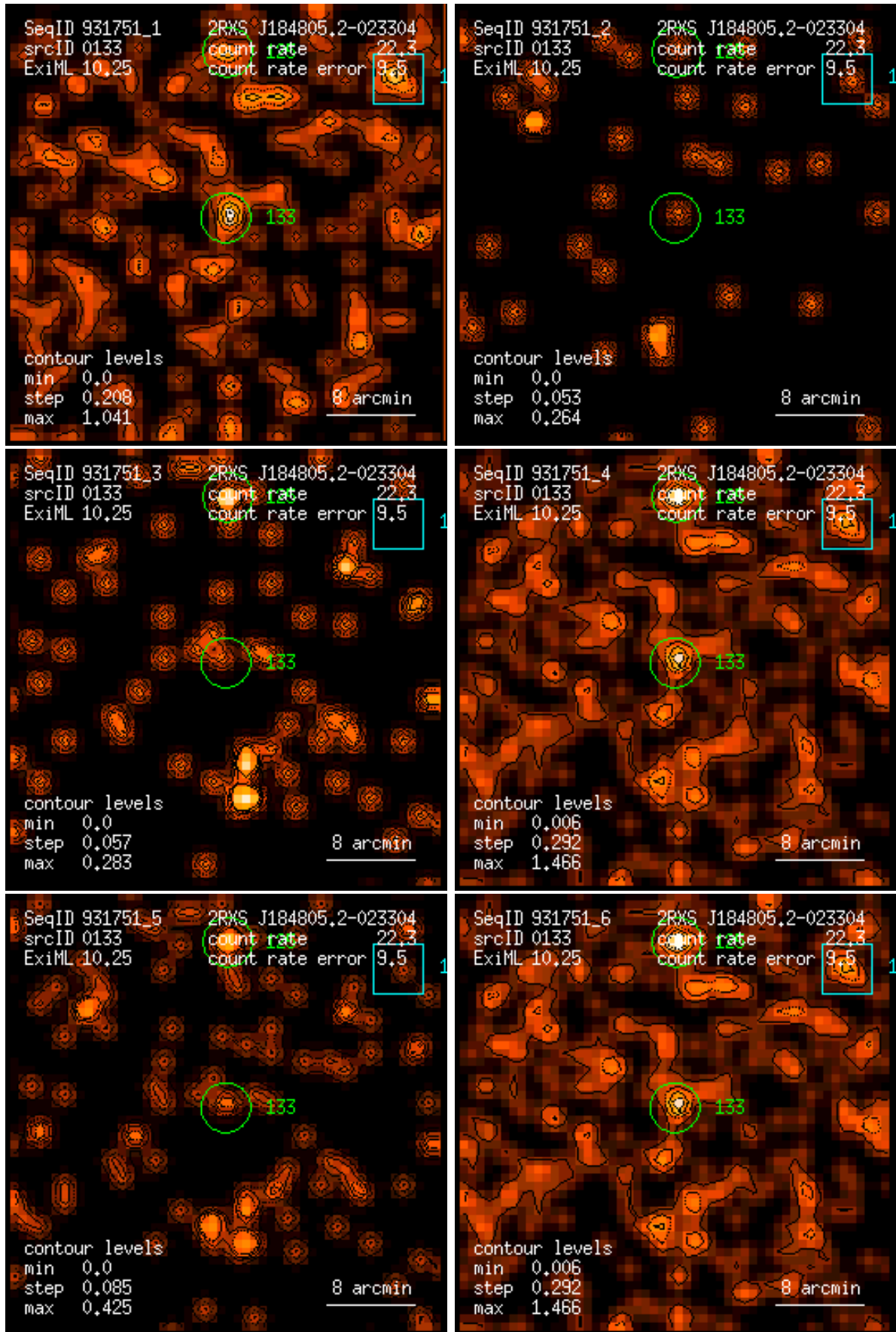
Figure 133: RASS 931751: detection 0133: band rate images, Gaussian filter: (1) PSPC channels 11 – 41, (2) 52 – 90, (3) 91 – 201, (4) 11 – 235, (5) 52 – 201, (6) 11 – 201. Broad band rates in counts/ks. Band rate contour levels in counts/ks/arcmin 2 .
