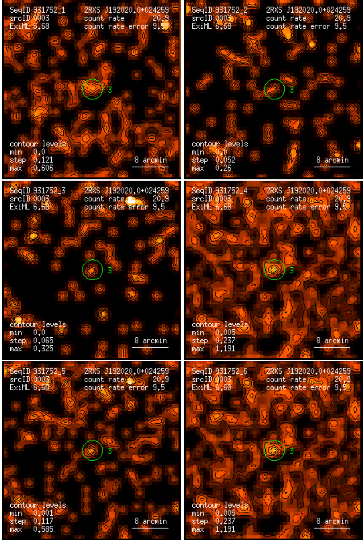
Figure 3: RASS 931752: detection 0003: band rate images, Gaussian filter: (1) PSPC channels 11 – 41, (2) 52 – 90, (3) 91 – 201, (4) 11 – 235, (5) 52 – 201, (6) 11 – 201. Broad band rates in counts/ks. Band rate contour levels in counts/ks/arcmin 2 .
