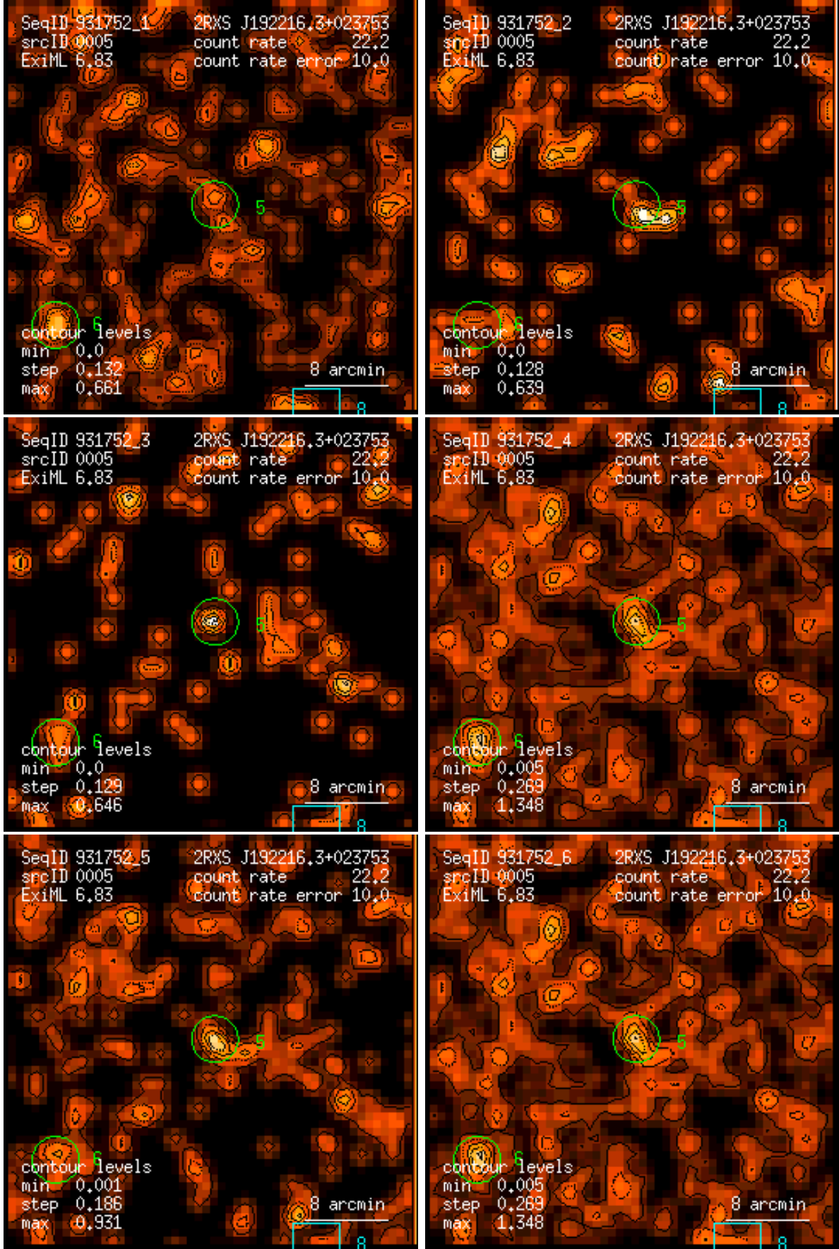
Figure 5: RASS 931752: detection 0005: band rate images, Gaussian filter: (1) PSPC channels 11 – 41, (2) 52 – 90, (3) 91 – 201, (4) 11 – 235, (5) 52 – 201, (6) 11 – 201. Broad band rates in counts/ks. Band rate contour levels in counts/ks/arcmin 2 .
