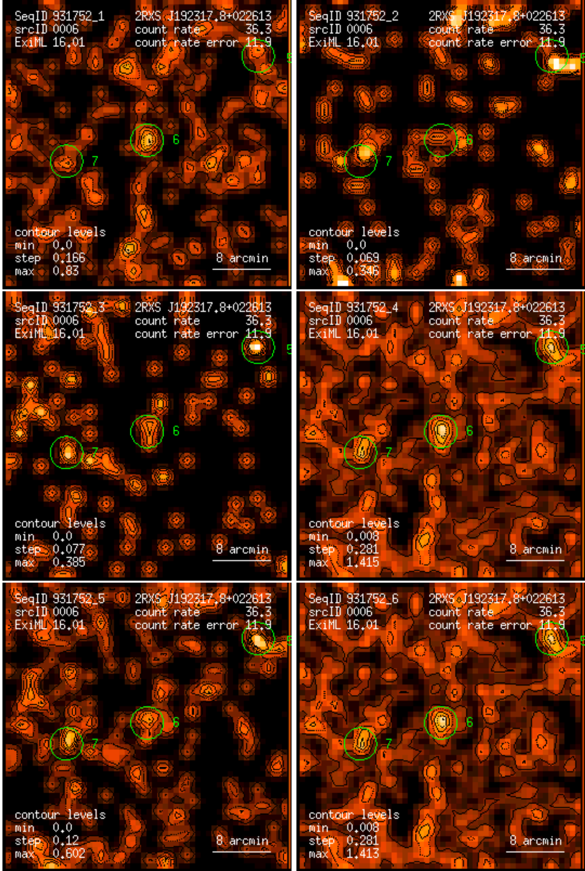
Figure 6: RASS 931752: detection 0006: band rate images, Gaussian filter: (1) PSPC channels 11 – 41, (2) 52 – 90, (3) 91 – 201, (4) 11 – 235, (5) 52 – 201, (6) 11 – 201. Broad band rates in counts/ks. Band rate contour levels in counts/ks/arcmin 2 .
