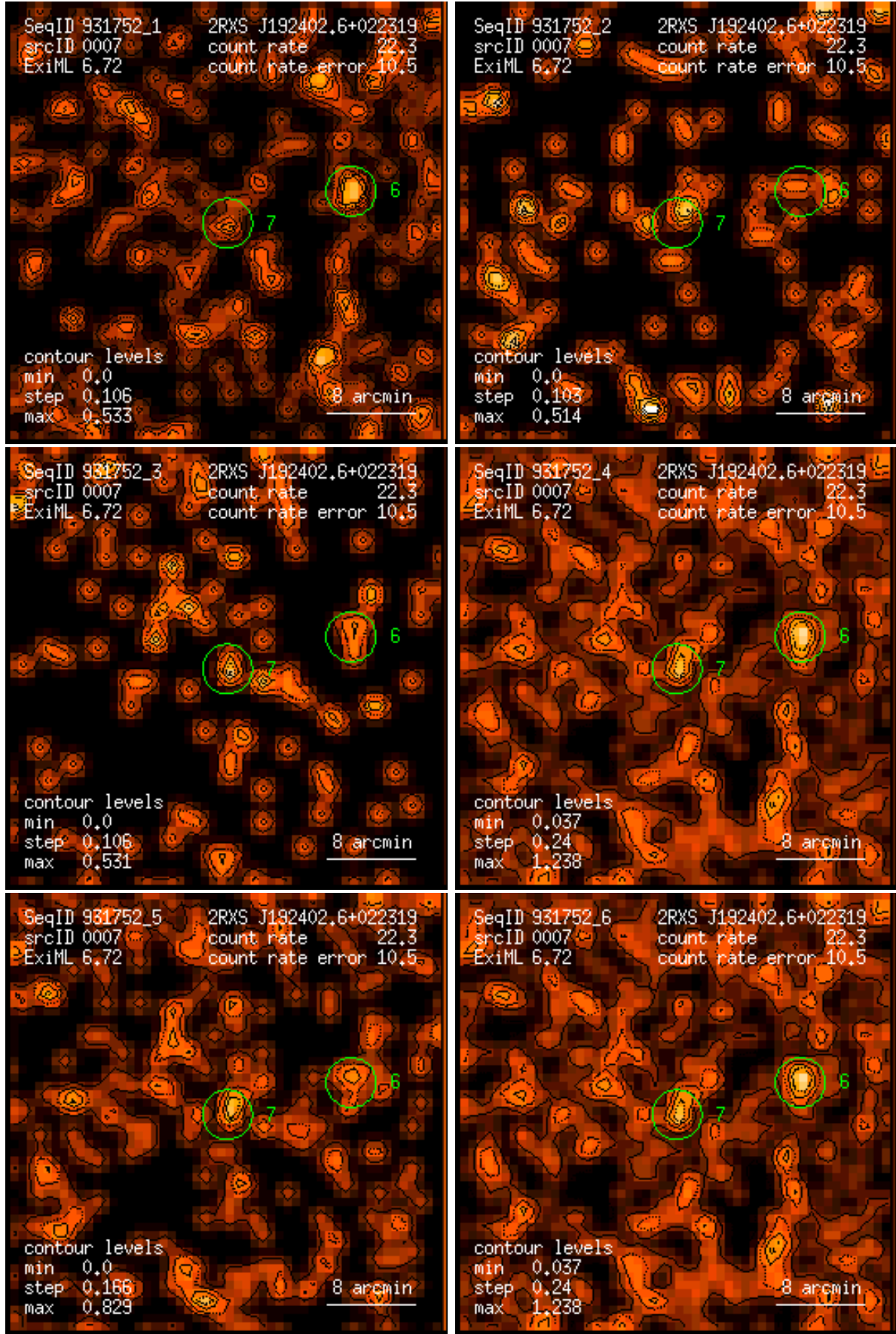
Figure 7: RASS 931752: detection 0007: band rate images, Gaussian filter: (1) PSPC channels 11 – 41, (2) 52 – 90, (3) 91 – 201, (4) 11 – 235, (5) 52 – 201, (6) 11 – 201. Broad band rates in counts/ks. Band rate contour levels in counts/ks/arcmin 2 .
