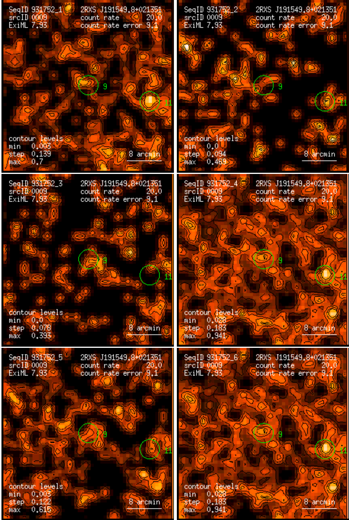
Figure 9: RASS 931752: detection 0009: band rate images, Gaussian filter: (1) PSPC channels 11 – 41, (2) 52 – 90, (3) 91 – 201, (4) 11 – 235, (5) 52 – 201, (6) 11 – 201. Broad band rates in counts/ks. Band rate contour levels in counts/ks/arcmin 2 .
