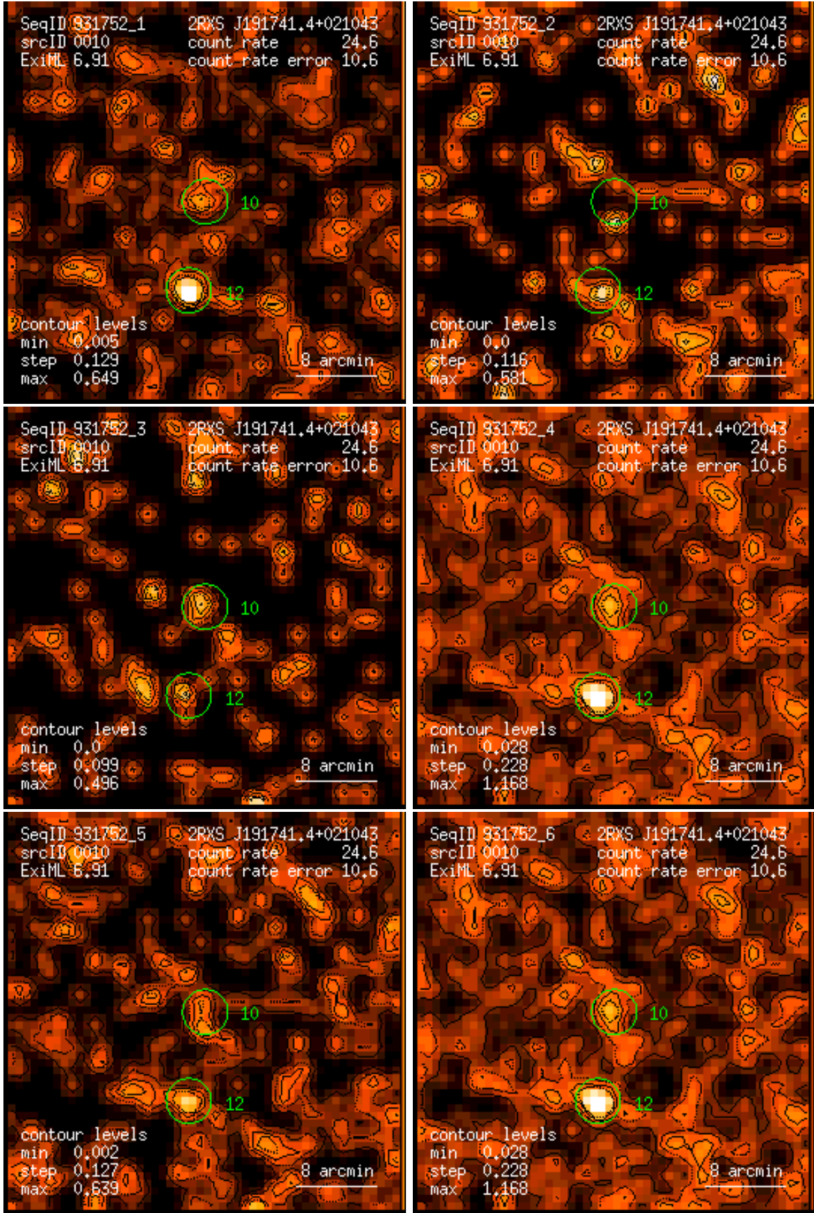
Figure 10: RASS 931752: detection 0010: band rate images, Gaussian filter: (1) PSPC channels 11 – 41, (2) 52 – 90, (3) 91 – 201, (4) 11 – 235, (5) 52 – 201, (6) 11 – 201. Broad band rates in counts/ks. Band rate contour levels in counts/ks/arcmin 2 .
