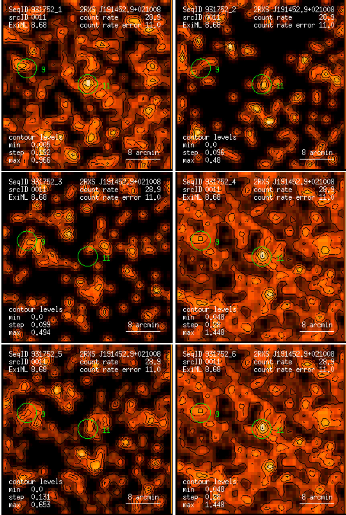
Figure 11: RASS 931752: detection 0011: band rate images, Gaussian filter: (1) PSPC channels 11 – 41, (2) 52 – 90, (3) 91 – 201, (4) 11 – 235, (5) 52 – 201, (6) 11 – 201. Broad band rates in counts/ks. Band rate contour levels in counts/ks/arcmin 2 .
