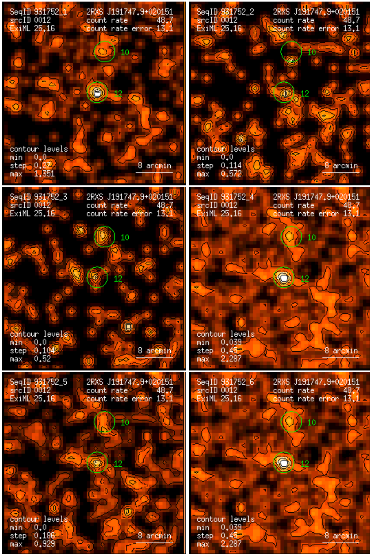
Figure 12: RASS 931752: detection 0012: band rate images, Gaussian filter: (1) PSPC channels 11 – 41, (2) 52 – 90, (3) 91 – 201, (4) 11 – 235, (5) 52 – 201, (6) 11 – 201. Broad band rates in counts/ks. Band rate contour levels in counts/ks/arcmin 2 .
