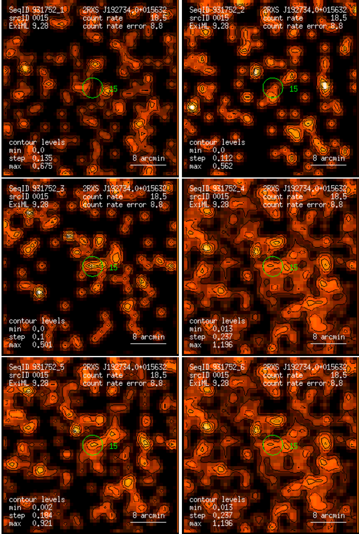
Figure 15: RASS 931752: detection 0015: band rate images, Gaussian filter: (1) PSPC channels 11 – 41, (2) 52 – 90, (3) 91 – 201, (4) 11 – 235, (5) 52 – 201, (6) 11 – 201. Broad band rates in counts/ks. Band rate contour levels in counts/ks/arcmin 2 .
