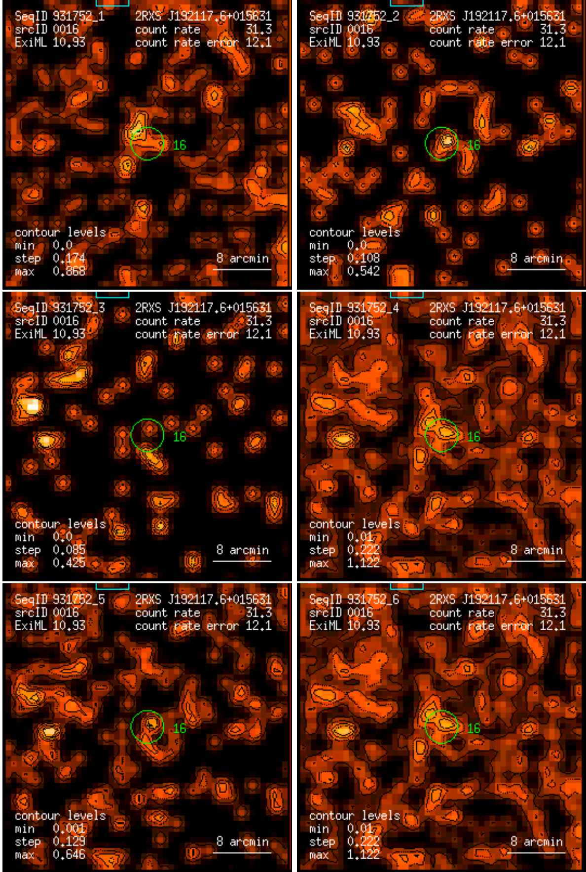
Figure 16: RASS 931752: detection 0016: band rate images, Gaussian filter: (1) PSPC channels 11 – 41, (2) 52 – 90, (3) 91 – 201, (4) 11 – 235, (5) 52 – 201, (6) 11 – 201. Broad band rates in counts/ks. Band rate contour levels in counts/ks/arcmin 2 .
