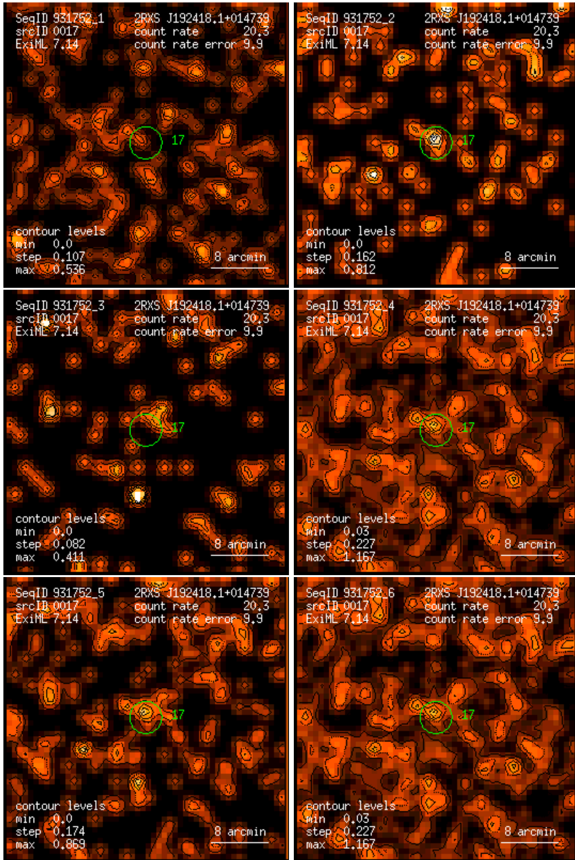
Figure 17: RASS 931752: detection 0017: band rate images, Gaussian filter: (1) PSPC channels 11 – 41, (2) 52 – 90, (3) 91 – 201, (4) 11 – 235, (5) 52 – 201, (6) 11 – 201. Broad band rates in counts/ks. Band rate contour levels in counts/ks/arcmin 2 .
