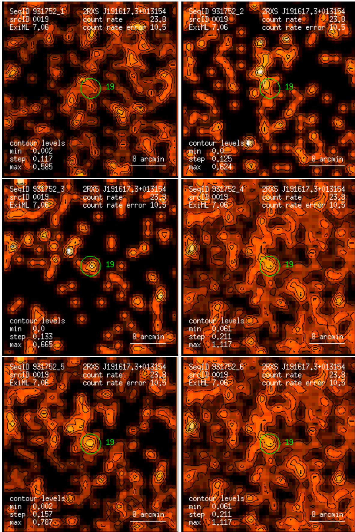
Figure 19: RASS 931752: detection 0019: band rate images, Gaussian filter: (1) PSPC channels 11 – 41, (2) 52 – 90, (3) 91 – 201, (4) 11 – 235, (5) 52 – 201, (6) 11 – 201. Broad band rates in counts/ks. Band rate contour levels in counts/ks/arcmin 2 .
