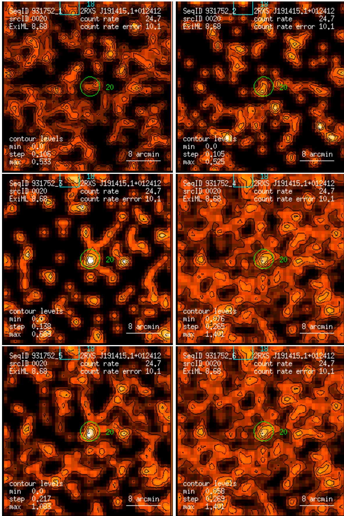
Figure 20: RASS 931752: detection 0020: band rate images, Gaussian filter: (1) PSPC channels 11 – 41, (2) 52 – 90, (3) 91 – 201, (4) 11 – 235, (5) 52 – 201, (6) 11 – 201. Broad band rates in counts/ks. Band rate contour levels in counts/ks/arcmin 2 .
