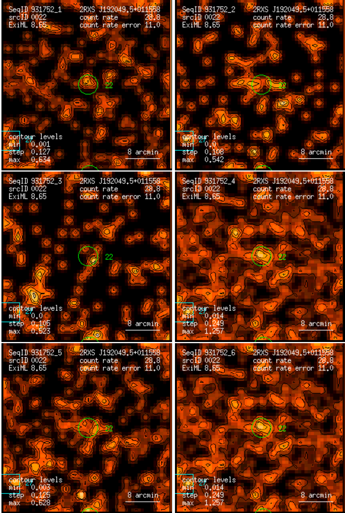
Figure 22: RASS 931752: detection 0022: band rate images, Gaussian filter: (1) PSPC channels 11 – 41, (2) 52 – 90, (3) 91 – 201, (4) 11 – 235, (5) 52 – 201, (6) 11 – 201. Broad band rates in counts/ks. Band rate contour levels in counts/ks/arcmin 2 .
