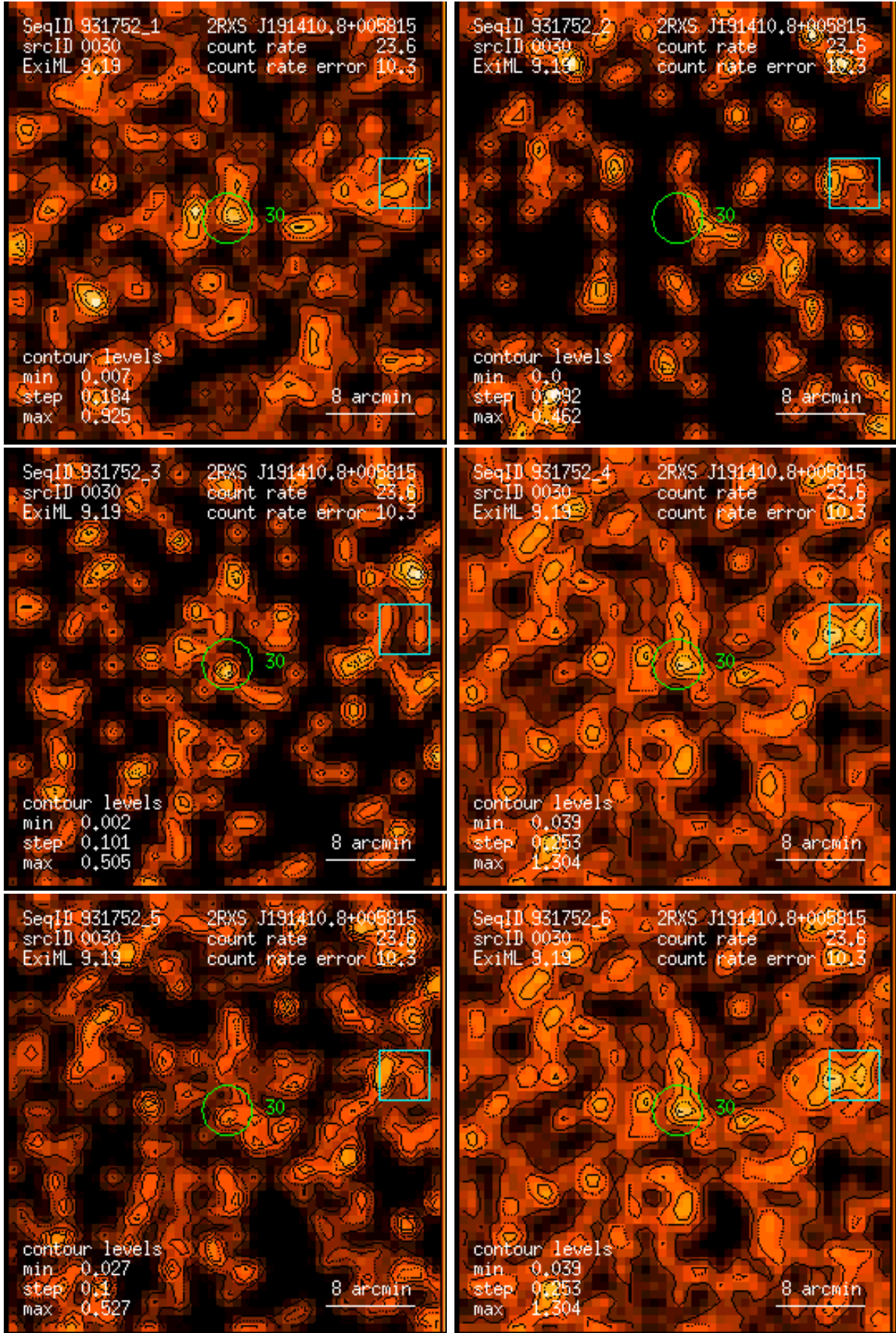
Figure 30: RASS 931752: detection 0030: band rate images, Gaussian filter: (1) PSPC channels 11 – 41, (2) 52 – 90, (3) 91 – 201, (4) 11 – 235, (5) 52 – 201, (6) 11 – 201. Broad band rates in counts/ks. Band rate contour levels in counts/ks/arcmin 2 .
