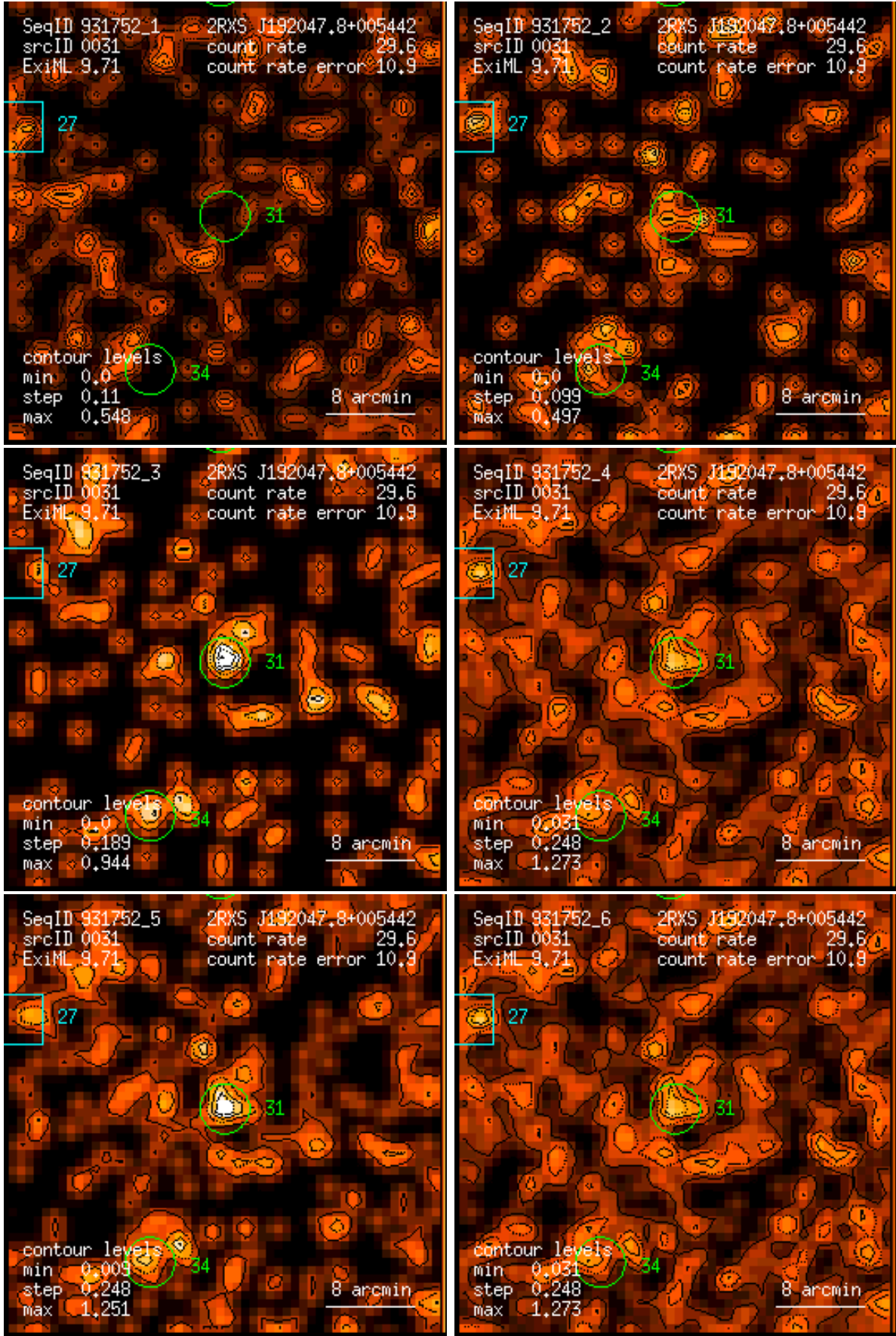
Figure 31: RASS 931752: detection 0031: band rate images, Gaussian filter: (1) PSPC channels 11 – 41, (2) 52 – 90, (3) 91 – 201, (4) 11 – 235, (5) 52 – 201, (6) 11 – 201. Broad band rates in counts/ks. Band rate contour levels in counts/ks/arcmin 2 .
