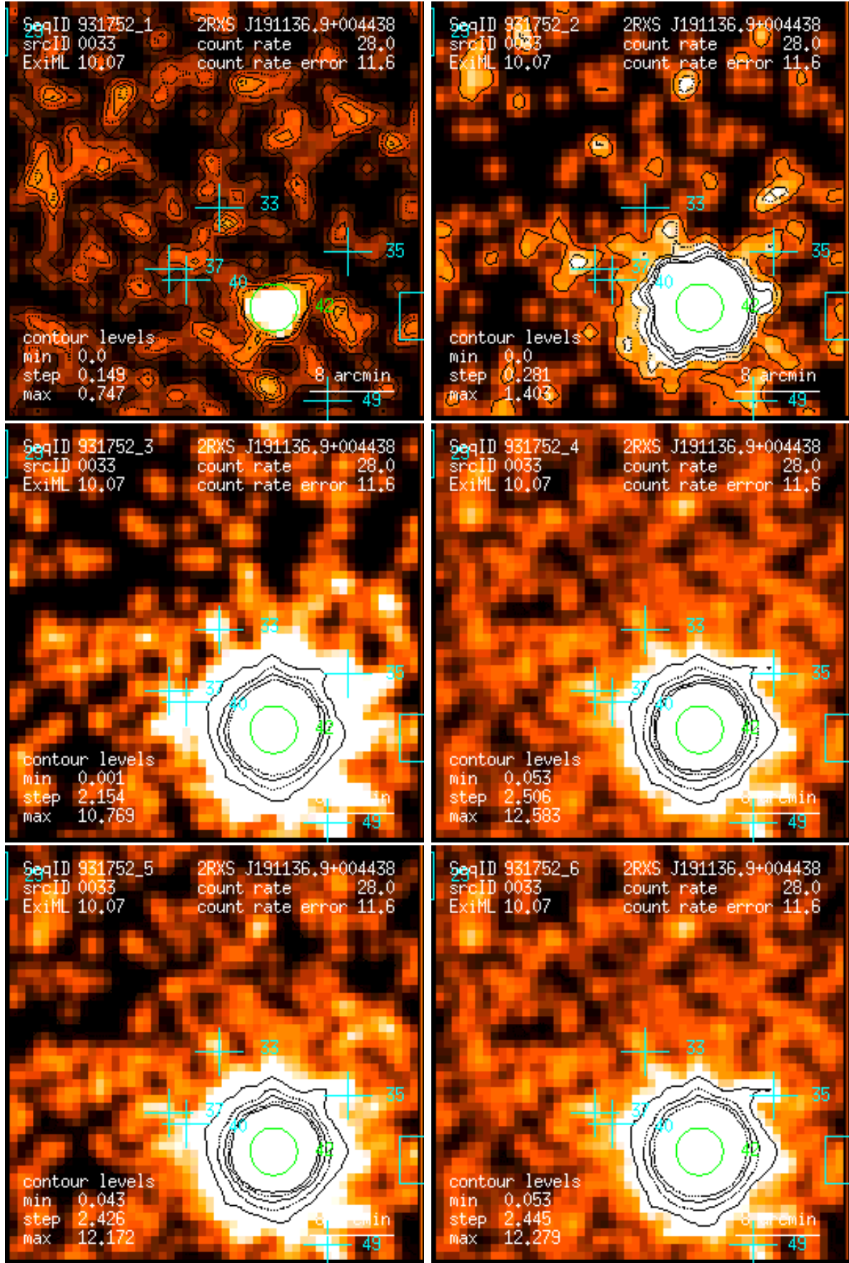
Figure 33: RASS 931752: detection 0033: band rate images, Gaussian filter: (1) PSPC channels 11 – 41, (2) 52 – 90, (3) 91 – 201, (4) 11 – 235, (5) 52 – 201, (6) 11 – 201. Broad band rates in counts/ks. Band rate contour levels in counts/ks/arcmin 2 .
