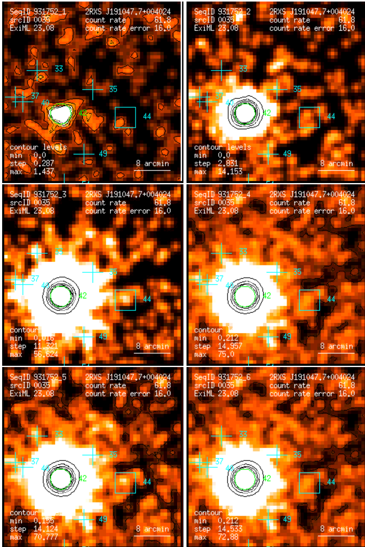
Figure 35: RASS 931752: detection 0035: band rate images, Gaussian filter: (1) PSPC channels 11 – 41, (2) 52 – 90, (3) 91 – 201, (4) 11 – 235, (5) 52 – 201, (6) 11 – 201. Broad band rates in counts/ks. Band rate contour levels in counts/ks/arcmin 2 .
